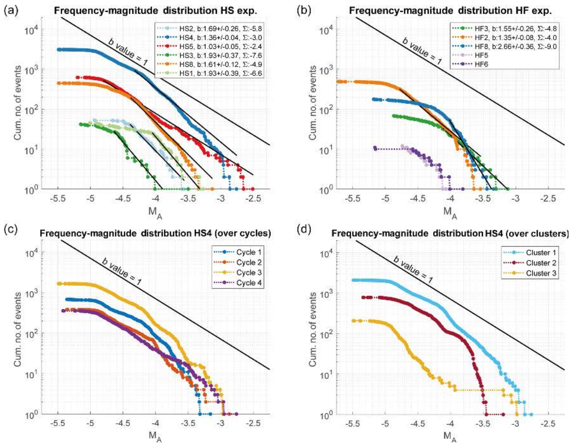
Figure 10. Frequency–magnitude distributions for the (a) HS and the (b) HF injection experiments along with estimated b values and seismogenic indices. Injection experiments in legends are ordered in a chronological manner, whereby HS injection experiments were performed in February 2017, and HF injection experiments were executed in May 2017. Frequency–magnitude distributions for injection experiment HS4, resolved in (c) injection cycles (Cycle 1–Cycle 4) and (d) clusters, introduced in Sect. 4.2. Uncertainties in b values are estimated after Marzocchi and Sandri (2009).
