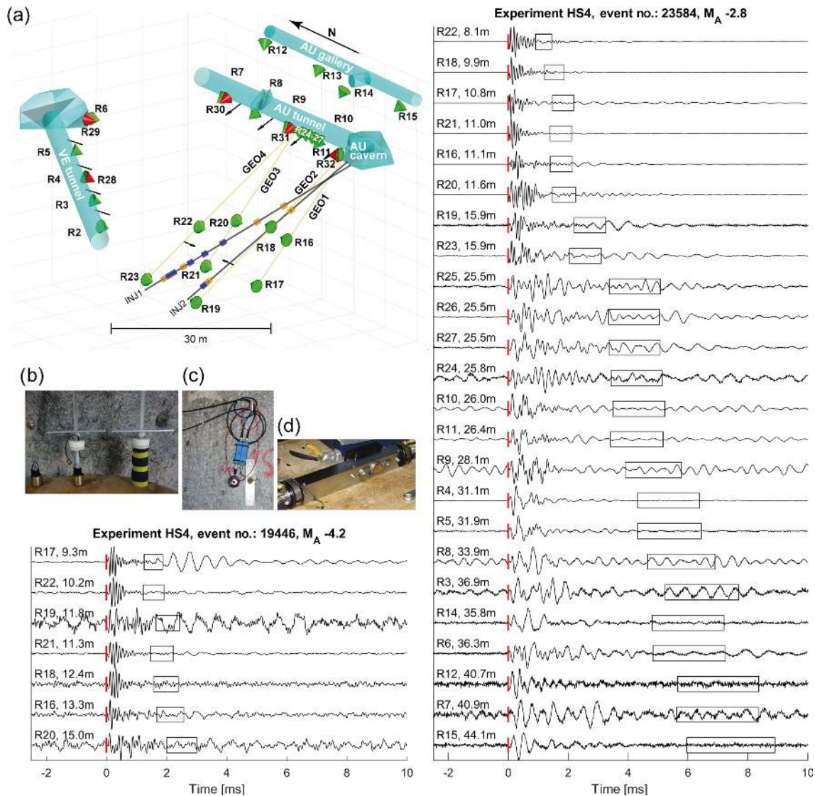
Figure 3. (a) The seismic network consisting of 26 uncalibrated AE sensors (green cones) installed in four boreholes, the AU and VE tunnels, and the AU gallery, along with five one-component calibrated accelerometers (red cones) collocated with five AE sensors in the AU and VE tunnels. Seismic sources in the tunnels and boreholes are shown by black arrows. (b) AE tunnel sensor, insulated against acoustic noise. (c) Installed AE sensor next to a calibrated accelerometer along with their pre-amplifiers. (d) AE sensors in a sensor shuttle for deployment into water-filled boreholes. Waveforms from a small- and large-magnitude event induced during experiment HS4, including the Euclidean distance hypocenter–sensor, P-wave pick (red-stripe), and a window of a hypothetical S-wave arrival for an S-wave velocity of 2500–3000 m s^{-1} (applied bandpass filter for small event: 1–12 kHz; large event: 1–50 kHz).
