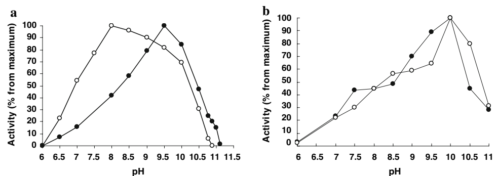
Fig. 4 Effect of pH on the activity of thiosulfate respiration in washed cells of ALCO 1 grown in batch (a) or continuous (b) culture at 2 M total Na + . Open symbols, cells grown in NaCl at pH 7.5; closed symbols, cells grown in soda at pH 10–10.05
