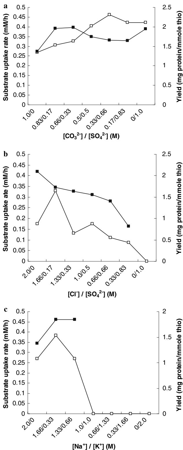
Fig. 6 Effect of replacement of CO 3 2- by SO 4 2- (a) at pH 10, Cl - by SO 4 2- (b) at pH 8, and Na + by K + (c) at pH 10, on substrate uptake rate (open symbols) and growth yield (closed symbols) in batch culture of strain ALCO 1 grown at 2 M of total cations and 2 M of total (monovalent) anions. As an inoculum, cells of ALCO 1 strain grown in continuous culture at pH 7.5 ( D = 0.033 h -1 ) and 10.05 ( D = 0.052 h -1 ), respectively, were used
