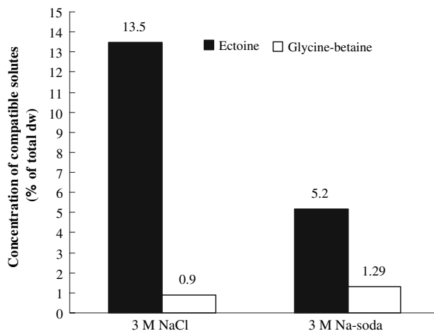
Fig. 7 Compatible solutes in the cells of ALCO 1 grown at 3 M total Na + and at different pH
