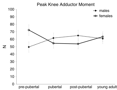
FIGURE 3 —Nonnormalized peak knee adductor moment during weight acceptance. Individual group data stratified by sex and maturation. Data represent mean + SE.
