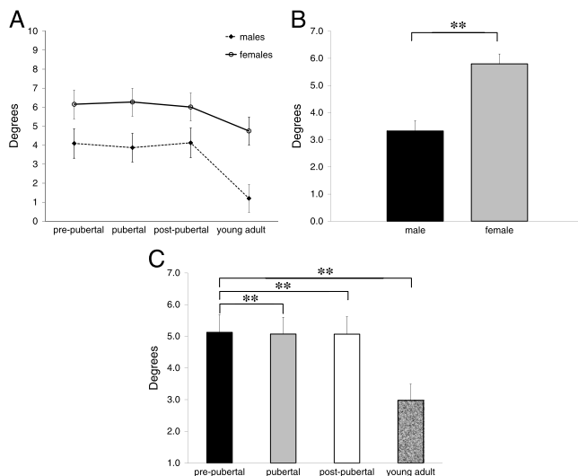
FIGURE 4 —Peak knee abductor angle ( ^{\circ} ) during weight acceptance. A, Individual group data stratified by sex and maturation. B, Data collapsed across sex. C, Data collapsed across maturation levels. Data represent mean + SE. **P \leq 0.01 .
