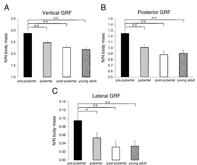
FIGURE 5 —Peak GRFs during weight acceptance (N/N body mass). Data are collapsed across sex. A, Vertical. B, Posterior. C, Lateral. Data represent mean + SE. *P < 0.05 ; **P \leq 0.01 .
