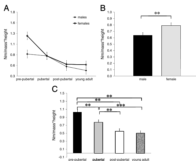
FIGURE 2—Peak knee adductor moment (N·m / mass \times height during weight acceptance. A, Individual group data stratified by sex and maturation. B, Data collapsed across sex. C, Data collapsed across maturation levels. Data represent mean \pm SE. ** P \leq 0.01 . N/N body mass, newtons of force / newtons of body mass.
