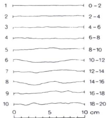
Fig. 2: Typical roughness profiles for JRC ranges [20].
