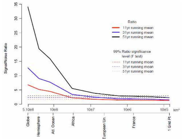
Fig. 5. Signal-Noise Ratio (SNR) calculated as a function of the spatial scale with the ratio of variance between the temperature in SGI and the CTRL described in Sect. 4. On the upper x-axis is the extent of the surface associated with the SNR. The lower x-axis gives references of geographic dimensions. The black, blue and red lines represent the SNR calculated with temperature time series smoothed with a 51, 31 and 11 yr running mean respectively. The black, blue and red dashed lines represent the 99th quantile of the Fisher distribution with 17, 28 and 85 degrees of freedom (dof) equivalent to the number of dof of a 850-year long time series smoothed with 51, 31 and 11 yr-running mean, respectively.
