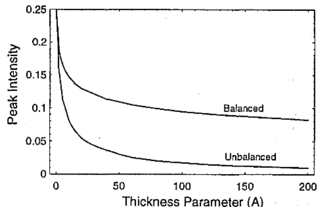
Fig. 6. Optimum peak intensity as a function of A for unbalanced and balanced cases.
