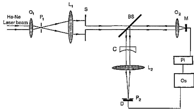
Fig. 8. Experimental setup: O_1 , O_2 , objectives; L_1 , L_2 , lenses; C , correction lens; P_1 , P_2 , pinholes; D , detector; BS , beam splitter; S , diaphragm; M , mirror acting as an object; O_s , oscilloscope; P_i , piezodriver.
