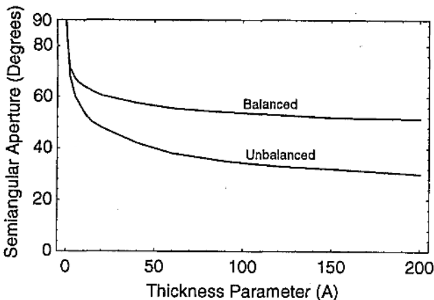
Fig. 4. Optimum semiangular aperture as a function of A for unbalanced and balanced cases.
