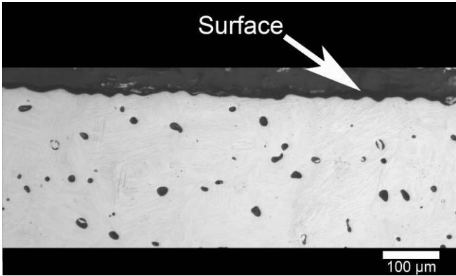
Fig. 12. Surface quality of MIM35H samples
