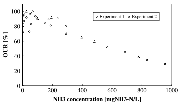
Figure 7. Process kinetics expressed as a percentage of OUR_{max} and NH_3 concentration ( 35^\circ C and pH = 8 ) showing inhibition of the nitrification kinetics at high NH_3 concentrations.
