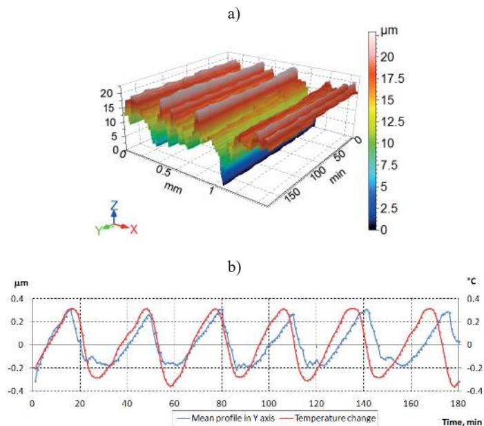
Fig. 14. Measurement results of ZERODUR® sample: a) isometric view, b) relationship between the profile in Y axis and temperature changes: P_t = 0,687 \mu\text{m} , \Delta t = 0.35^\circ\text{C}
