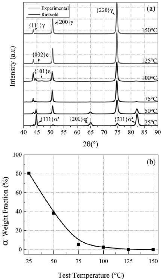
Figure 3. (a) XRD patterns (gray lines) and Rietveld refinement analysis (black lines) for the AISI 304 steel samples after strained up to UTS at 25, 50, 75, 100, 125 and 150°C. Austenite peaks are identified by \gamma , \alpha' martensite peaks by \alpha' and \epsilon martensite peaks by \epsilon . (b) \alpha' weight fraction as a function of test temperature.
