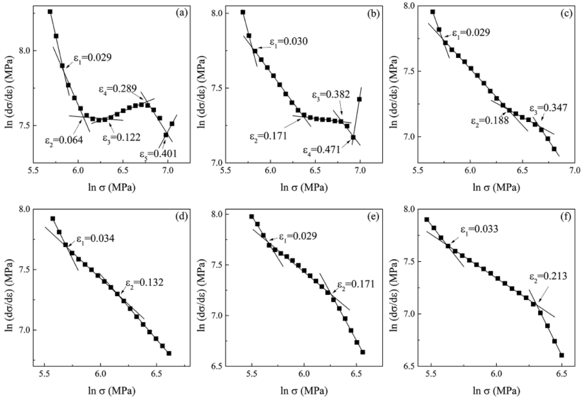
Figure 7. \ln(d\sigma/d\epsilon) vs. \ln(\sigma) plots for strain hardening stages distinction via modified C-J analysis of AISI 304 steel samples strained at 25°C (a), 50°C (b), 75°C (c), 100°C (d), 125°C (e) and 150°C (f).
