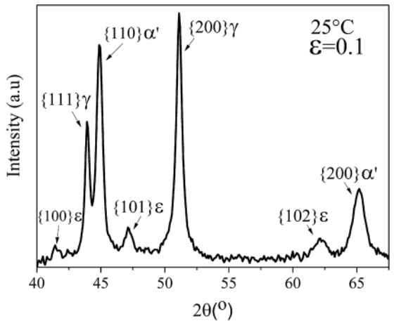
Figure 4. XRD pattern of AISI 304 steel sample after strained to \epsilon = 0.1 at 25°C. Intensity values are represented in a square root scale, in order to make the \{100\} , \{101\} and \{102\} \epsilon martensite reflections evident.
