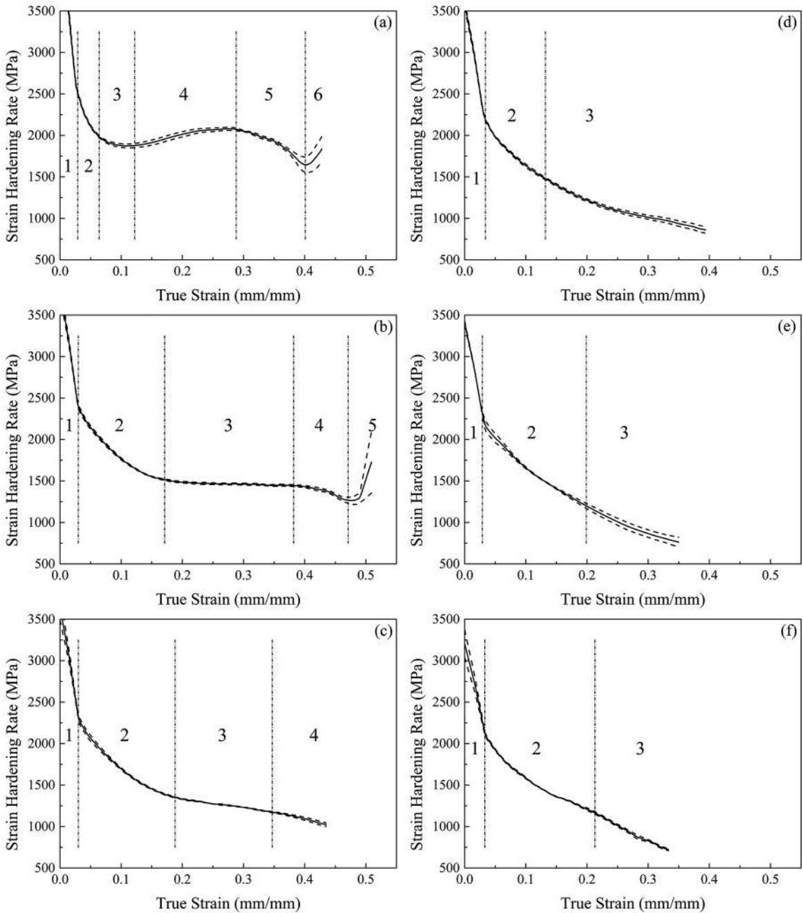
Figure 8. Strain hardening rate as a function of true strain of AISI 304 steel samples strained at 25°C (a), 50°C (b), 75°C (c), 100°C (d), 125°C (e) and 150°C (f).
