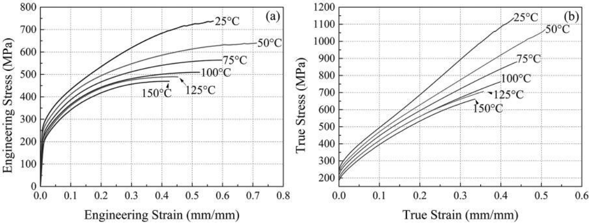
Figure 1. Engineering stress-strain curves (a) and flow curves (b) of a stainless AISI 304 steel strained at 25, 50, 75, 100, 125 and 150°C at a fixed strain rate of 10^{-3}\text{s}^{-1} .
