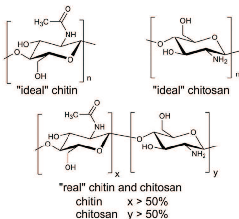
Fig. 1. The chemical structures of chitin and chitosan
