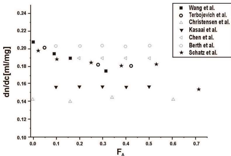
Fig. 2. Variation of the dn/dc values.
