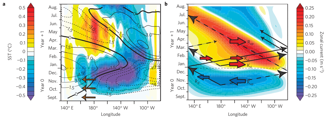
Figure 3 | Longitude-time diagram of equatorial ( 2^{\circ}\text{S} – 2^{\circ}\text{N} ) Pacific response to the IOD external forcing, as estimated from a shallow-water model experiment. a , Thermocline depth (contours, with negative values dashed; m) and SST (colours) anomalies. The arrows indicate the period at which the wind stress perturbation corresponding to IOD external forcing has been applied. b , Zonal current anomalies (colours). The Kelvin (K) and Rossby (R) wave response is indicated by thin black arrows (continuous line for downwelling (d) and dashed for upwelling (up) waves). The resulting zonal current perturbations are indicated by blue (westward) and red (eastward) arrows. The horizontal dashed line marks the transition from year 0 to year 1.
