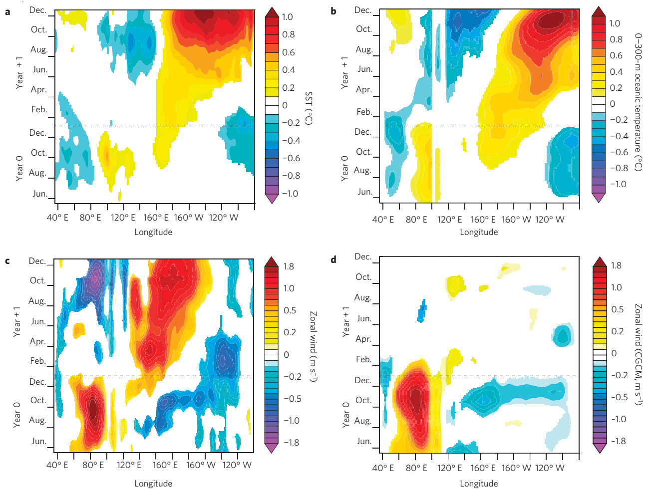
Figure 2 | Longitude-time section of Indo-Pacific anomalies associated with a negative IOD. a , Observed SST ( ^{\circ}\text{C} ). b , 0–300-m oceanic temperature ( ^{\circ}\text{C} ). c , Zonal wind ( \text{m s}^{-1} ) over the Indo-Pacific during and after a negative IOD event (the influence of ENSO has been removed, see the Methods section). d , Indo-Pacific zonal wind signals associated with the IOD in a coupled model experiment with no coupling over the tropical Pacific. Signals are within 2^{\circ}\text{S} – 2^{\circ}\text{N} , except for SST (within 5^{\circ}\text{S} – 5^{\circ}\text{N} in the Pacific, and 10^{\circ}\text{S} – 0^{\circ}\text{N} to the west of 120^{\circ}\text{E} ). Only signals significant at the 90% level are plotted. The dashed line marks the transition from year 0 to year 1.
