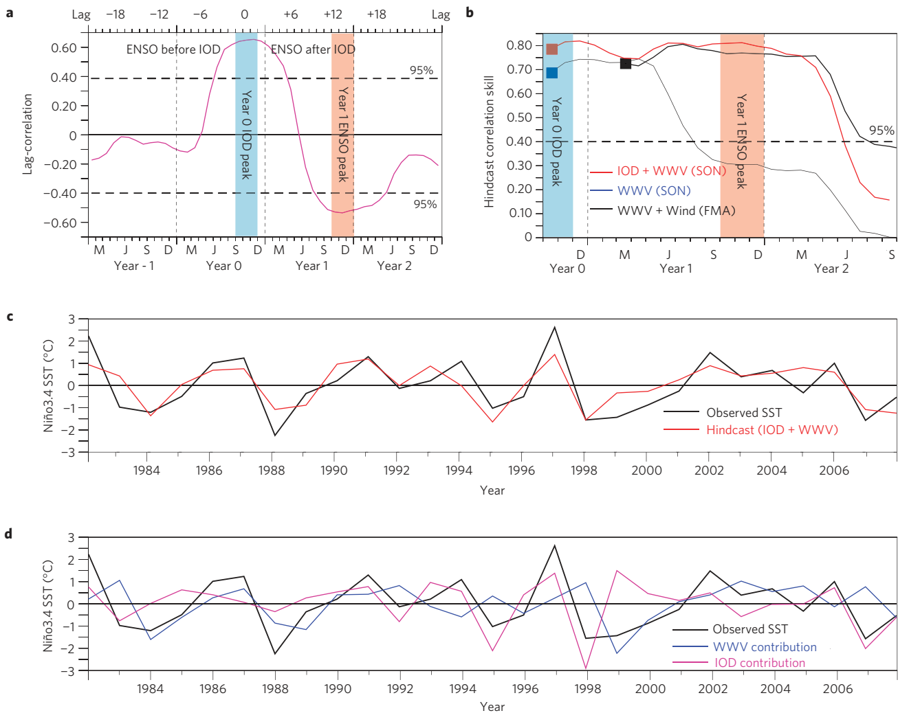
Figure 1 | IOD index as a precursor of the following year's ENSO state. a , Lag-correlation between IOD (in September–November of year 0) and ENSO indices (dashed lines indicate the 95% confidence limit). b , Correlation skill of Niño3.4 SST hindcasts using WWV and western Pacific zonal wind in February–April of year 1 (black), using only WWV in September–November of year 0 (blue), or WWV + IOD index in September–November of year 0 (red). c , Observed (black) and predicted (red) ENSO index using the WWV and IOD indices of September–November 13 months before. d , Black curve as in c ; the hindcast in c (red) is the sum of the WWV (blue) and DMI (purple) contributions shown in d .
