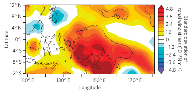
Figure 4 | Intraseasonal zonal wind stress variations in the western Pacific in December–March after a negative IOD. Standard deviation of 30–100 days' band-pass-filtered zonal wind stress in DJFM partially regressed to minus the IOD index, with the ENSO influence removed ( 10^{-3}\text{ N m}^{-2} , 90% significance level in black contours).
