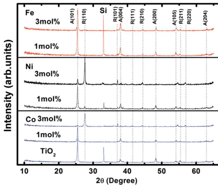
Figure 5 XRD patterns of undoped and TM-doped \text{TiO}_2 films.
