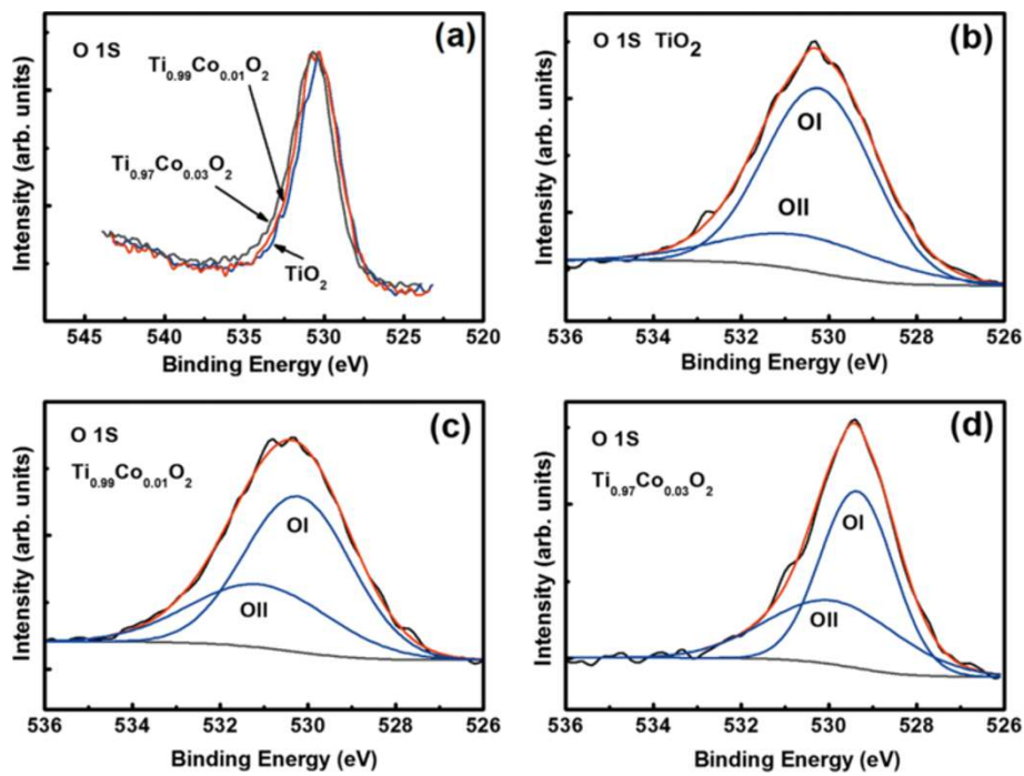
Figure 4 Normalized and fitted XPS core level spectra of oxygen 1s level. Normalized XPS core level spectra of oxygen 1s level of undoped and Co-doped \text{TiO}_2 (a). Fitted XPS core level spectra of oxygen 1s level of \text{TiO}_2 film (b), \text{Ti}_{0.99}\text{Co}_{0.01}\text{O}_2 film (c), and \text{Ti}_{0.97}\text{Co}_{0.03}\text{O}_2 film (d).
