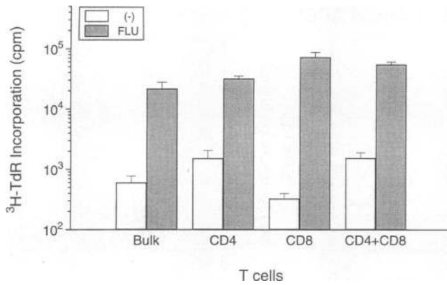
Figure 8. Purified CD4 + and CD8 + T cells proliferate to influenza virus-infected dendritic cells. CD4 + and CD8 + T cells were purified from a bulk T cell population to > 98% by staining with specific mAbs, followed by sorting on a FACStar Plus, as described in Methods. Bulk T cells, sorted CD4 + , CD8 + , and a combination of both sorted populations (CD4/CD8 cell ratio of 2:1) were tested in a standard proliferation assay for responsiveness to influenza virus-infected ER - , FcR - cells. The T/APC ratio was 5:1. Clear bars represent the responses to uninfected APCs whereas shaded bars represent the influenza virus-specific responses. Cultures were pulsed on day 5 for 12 h with 4 \mu Ci/ml of [ 3 H]TdR. Results are means of triplicates \pm SD. Note the log scale on the y-axis.
