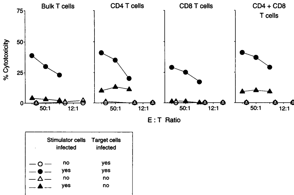
Figure 9. Dendritic cells stimulate the development of both CD4 + and CD8 + influenza virus-specific CTL. Bulk T cells and sorted purified CD4 + or CD8 + cells were stimulated with uninfected (open symbols) or infected (closed symbols) ER - , FcR - cells for 7 d. The T/APC ratio was 3:1. Cytolytic activity was measured on uninfected and infected syngeneic monocytes. CD4 + and CD8 + cells were also added together at a 2:1 ratio before the CTL assay (last panel on right).
