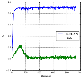
Figure 1: Lower bound L_I over training iterations
