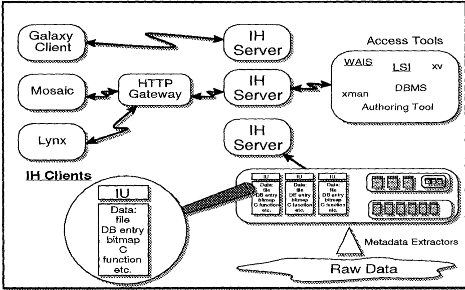
Fig. 3. InfoHarness Architecture.
