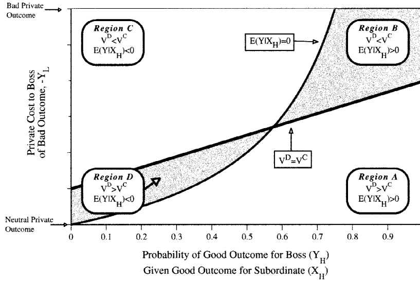
Figure 3. Relevant regions for analysis of decision authority when the boss is uninformed. The two lines depict all combinations of Y_L and \rho yielding V^D - V^C = 0 and E(Y|X_H) = \rho Y_H + (1 - \rho)Y_L = 0 .
