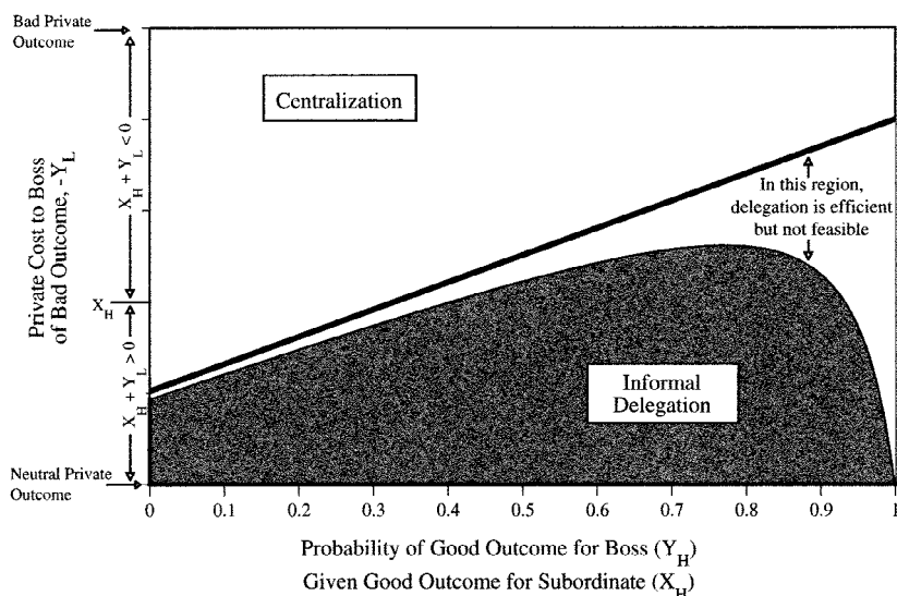
Figure 2. Relative efficiency of centralization and informal delegation for r > 0 and for different values of Y_L and p . The centralization region includes all combinations of Y_L and p yielding V^D - V^C < -rY_L ; informal delegation includes all combinations yielding V^D - V^C > -rY_L . Figure is drawn assuming X_H = Y_H and r = 30\% .
