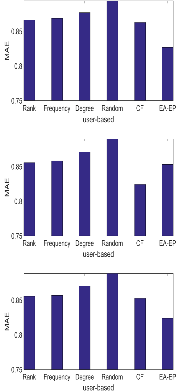
Fig.4 Results of MAE with 90,130,140 neighbors from different algorithms
