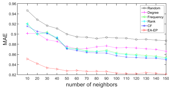
Fig.5 Comparison of average results of MAE in five cross validations with different number of neighbors in different algorithms
