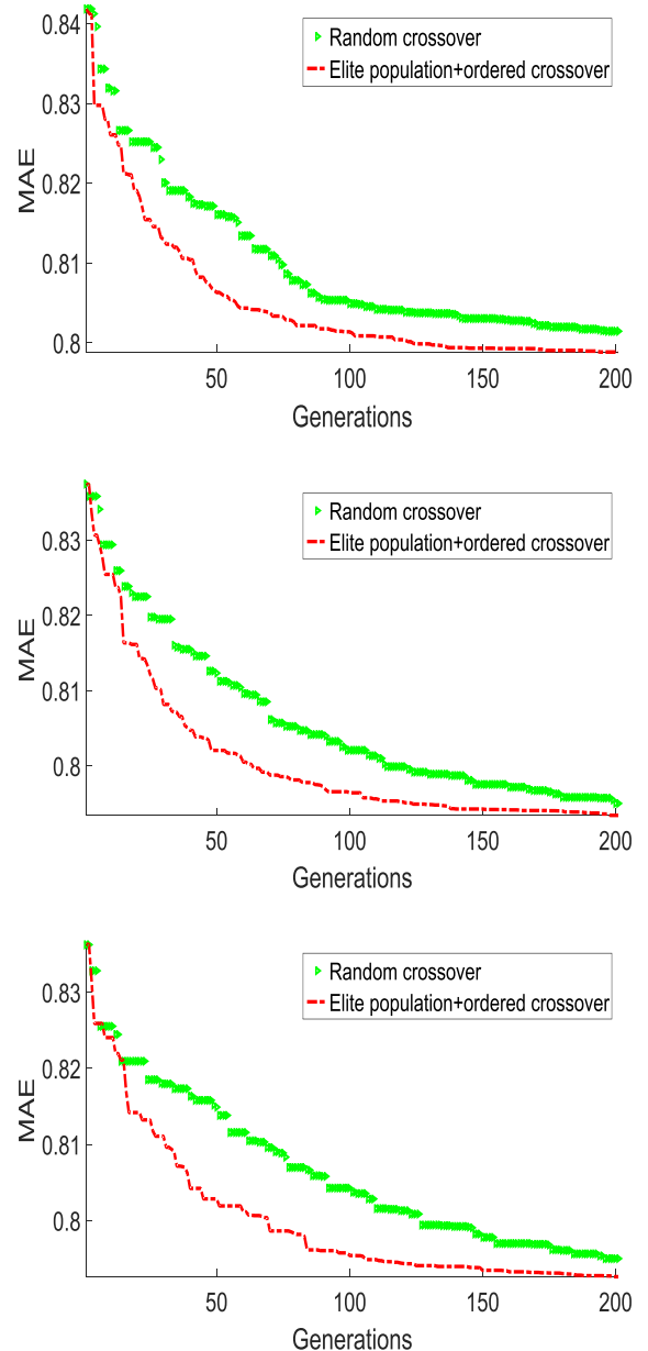
Fig.2 Comparisons between the random crossover and crossover with elitism in EA-EP with 90,130,140 neighborhoods
