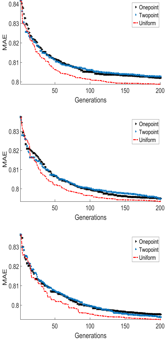
Fig.3 Comparisons between different crossover operators with 90,130,140 neighborhoods in EA-EP
