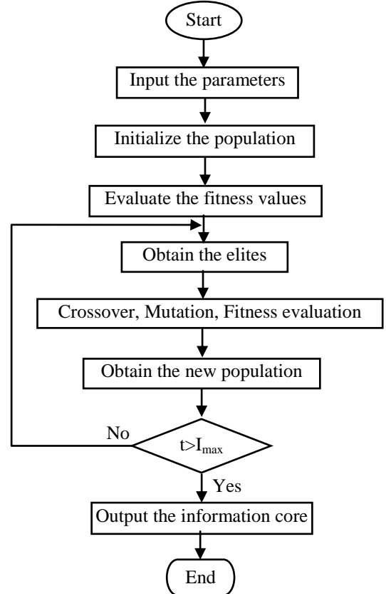
Fig.1 Flowchart of EA-EP
