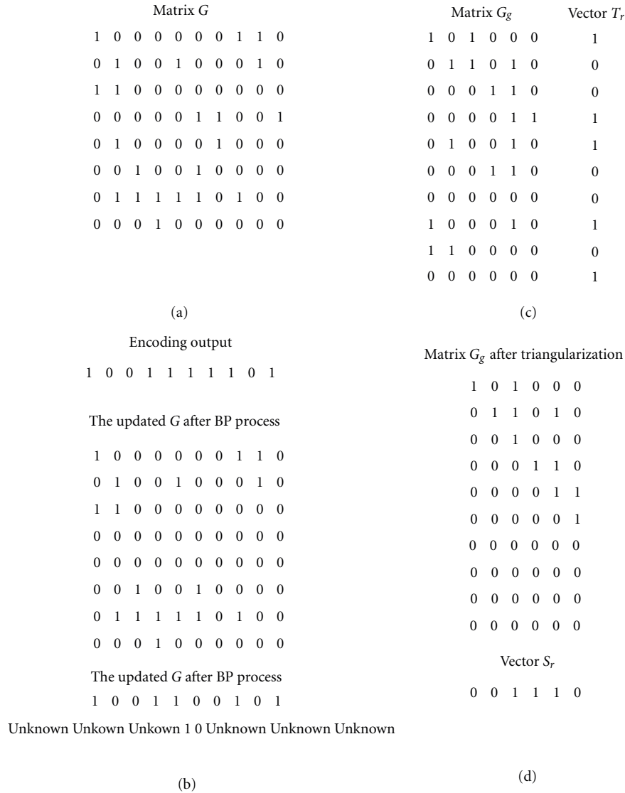
FIGURE 8: The original G matrix and the evolvement of G , T , and ST vector in the process of BGRA.
