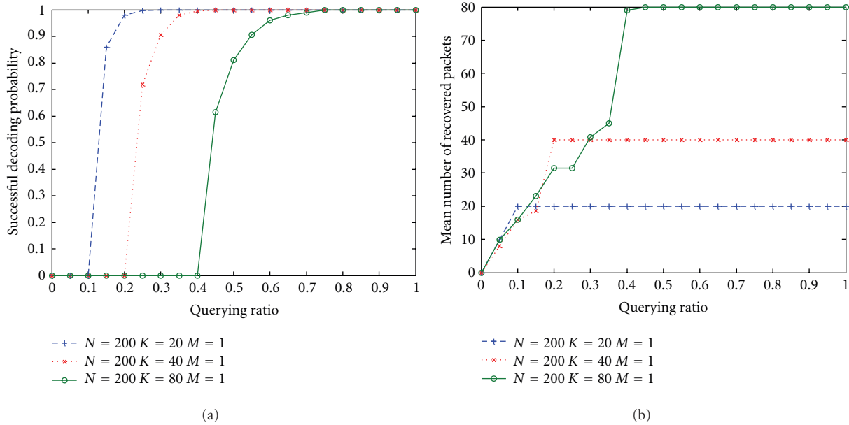
FIGURE 14: (a) The successful decoding performance; (b) the mean number of recovered packets as a function of querying ratio for networks with N = 200, M = 1 while the value of K/N changes.
