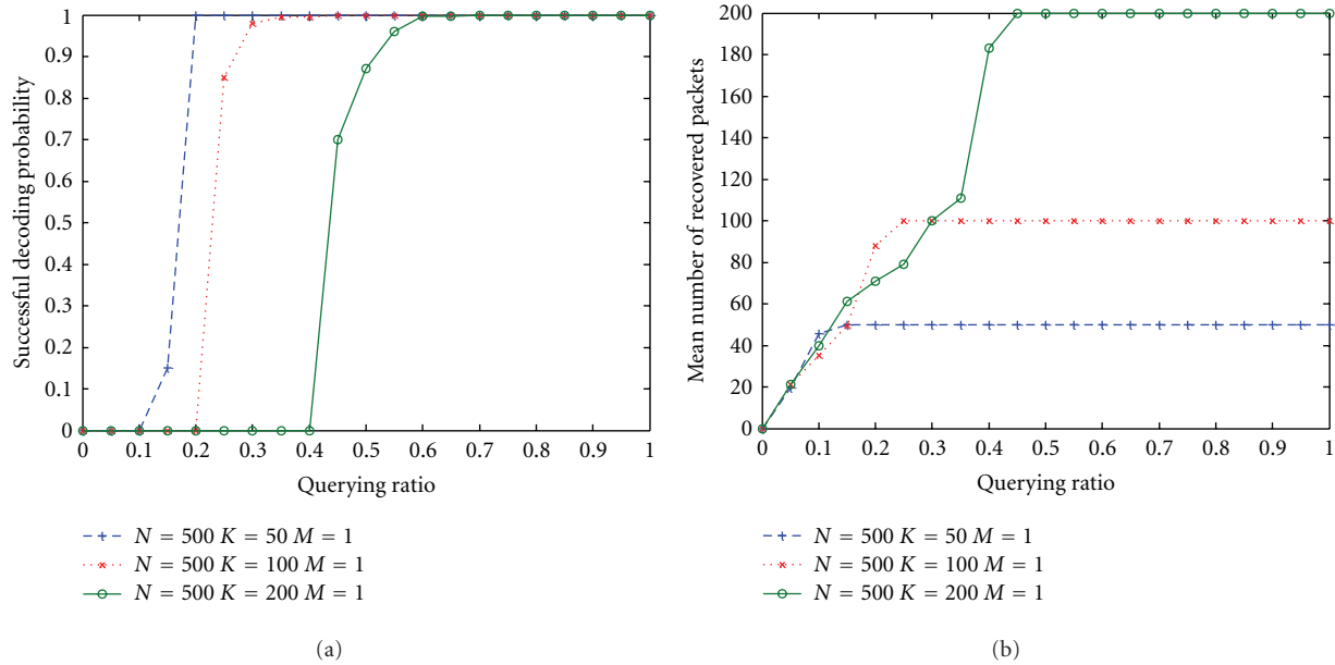
FIGURE 15: (a) The successful decoding performance; (b) the mean number of recovered packets as a function of querying ratio for networks with N = 500 , M = 1 while the value of K/N changes.
