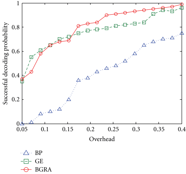
FIGURE 9: The successful decoding probability as a function of encoding overhead while k = 100 for LT code (0.01, 0.01).
