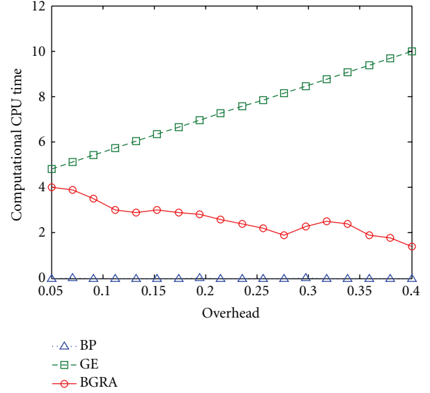
FIGURE 10: The computational CPU time as a function of encoding overhead while k = 100 for LT code (0.01, 0.01).
