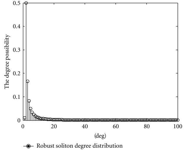
FIGURE 3: The Robust Soliton distribution \mu(0.01, 0.01) with k = 100 .
