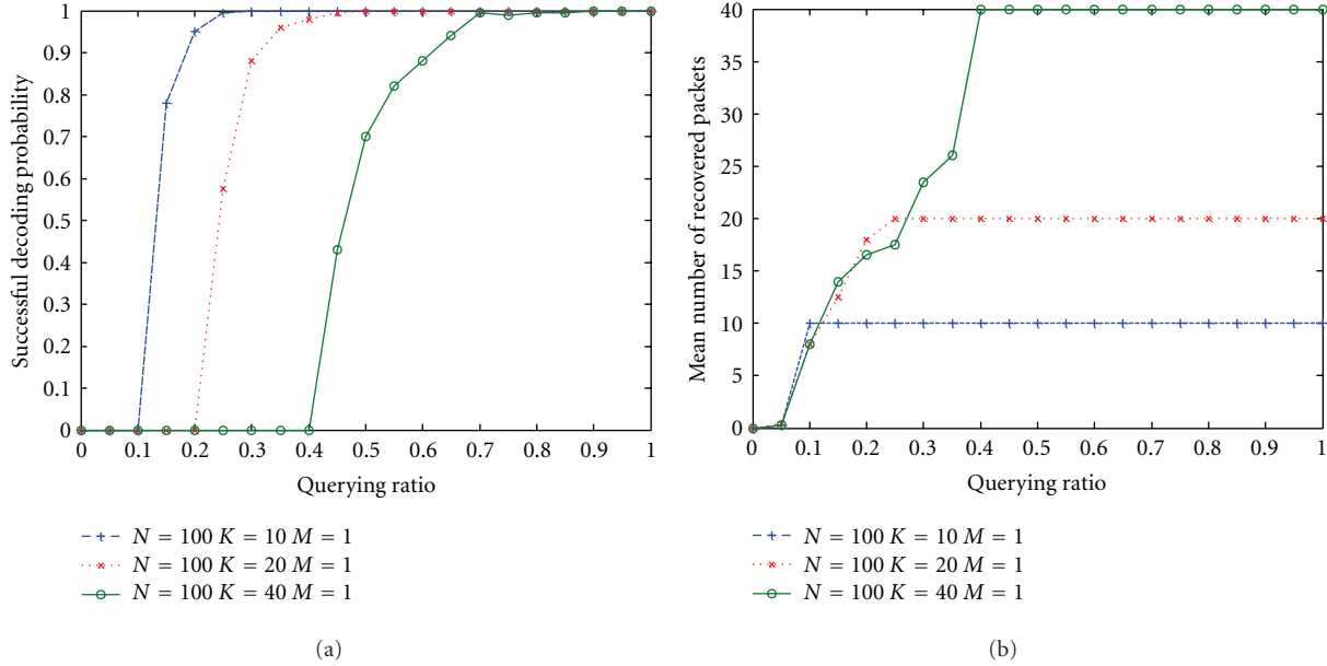
FIGURE 13: (a) The successful decoding performance; (b) the mean number of recovered packets as a function of querying ratio for networks with N = 100, M = 1 while the value of K/N changes.
