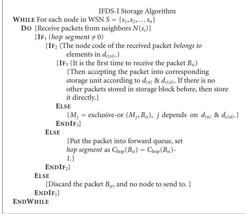
ALGORITHM 1: The algorithm flow of IFDS-I.
