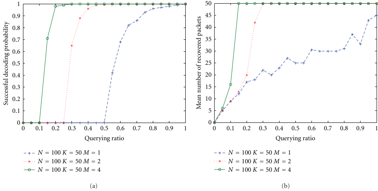
FIGURE 11: (a) The successful decoding performance; (b) the mean number of recovered packets as a function of querying ratio while N = 100 , K = 50 , K/N = 50\% , and M changes.
