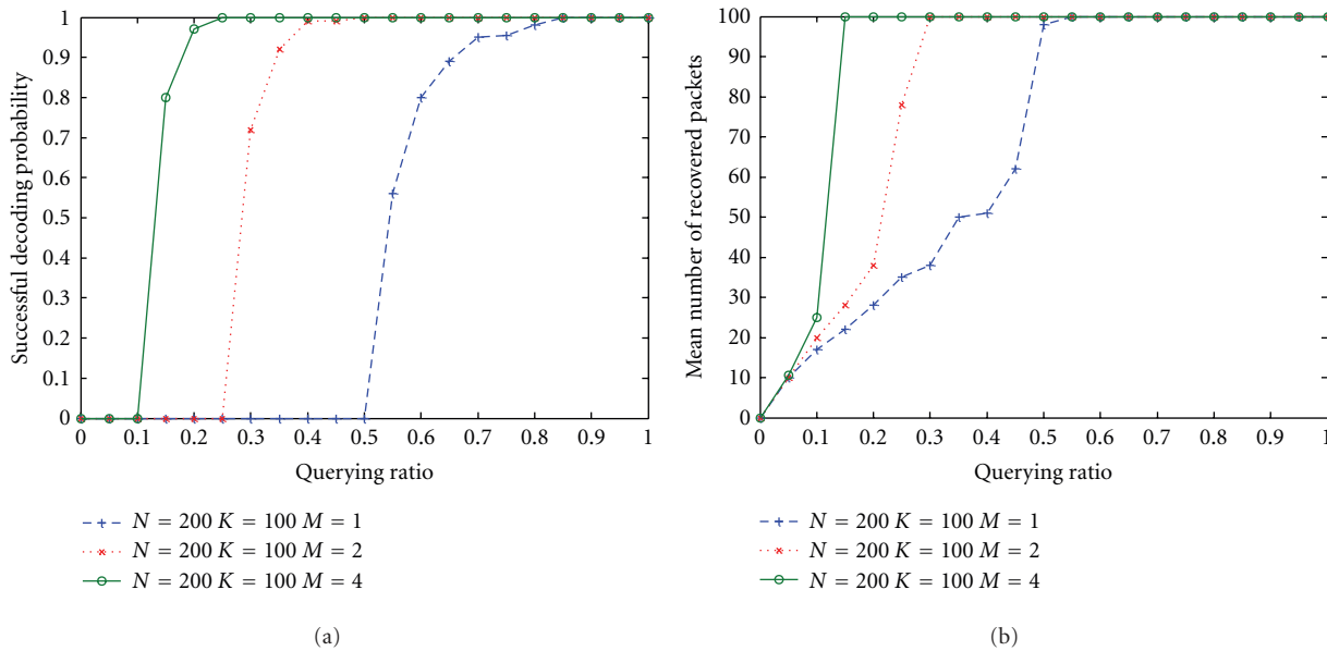
FIGURE 12: (a) The successful decoding performance; (b) the mean number of recovered packets as a function of querying ratio while N = 200 , K = 100 , K/N = 50\% , and M changes.
