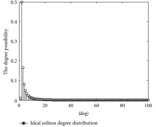
FIGURE 2: The Ideal Soliton degree distribution with k = 100 .
