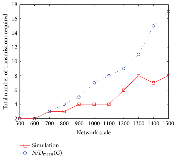
FIGURE 5: The relationship between network scale and C_{\text{hop}} .
