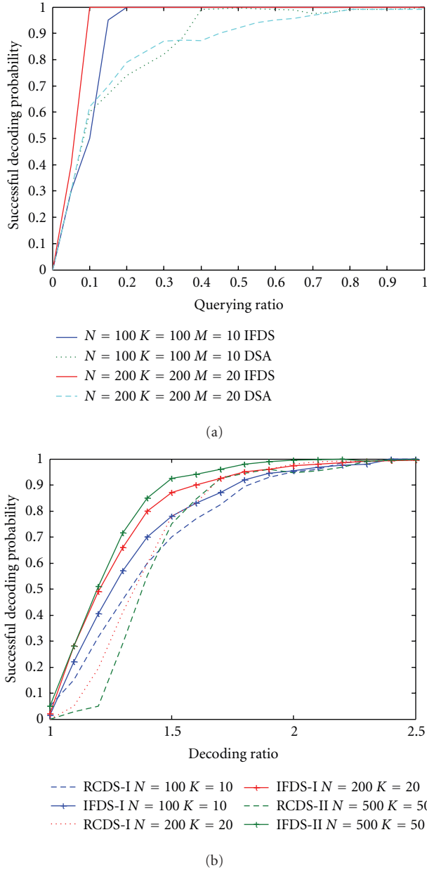
FIGURE 16: (a) Comparison of decoding performance using IFDS-I and DSA-I; (b) comparison of decoding performance using IFDS and RCDS.
