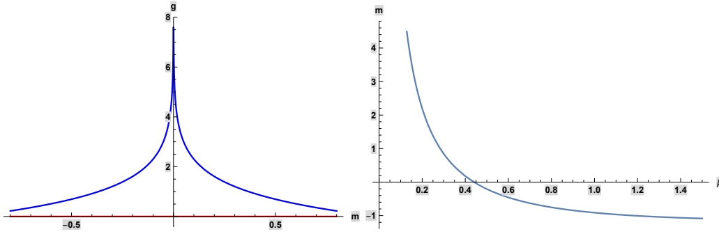
Figure 2: Left: real (blue) and imaginary (red) components of the Fisher information metric (44) for the 1d free fermion theory corresponding to the 2d classical Ising model. Note that the metric obtained via the mapping in [50] is only valid near the critical point m_c = 0 . Right: plot of the mass (46) as a function of \beta = \beta J = \beta K , from which we see that the free fermion mass vanishes precisely at the critical temperature (41), corresponding to the phase transition in the 2d model where one expects to find a conformal field theory. The mass also takes opposite signs on either side of the critical line in fig. 1 that matches the direction of divergence in the 2d curvature, i.e., we find m > 0 on the side nearer the origin and m < 0 on the side nearer \beta J = \beta K \rightarrow \infty .
