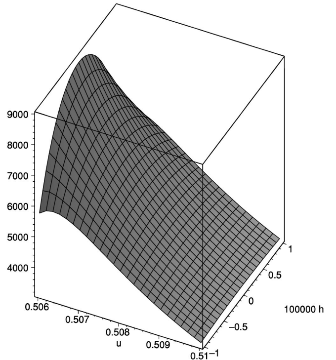
FIG. 1. A plot of \mathcal{R} close to u_{cr} = 1/2 . Note that the external field h is scaled by a factor of 10^5 and so covers a very narrow range.
