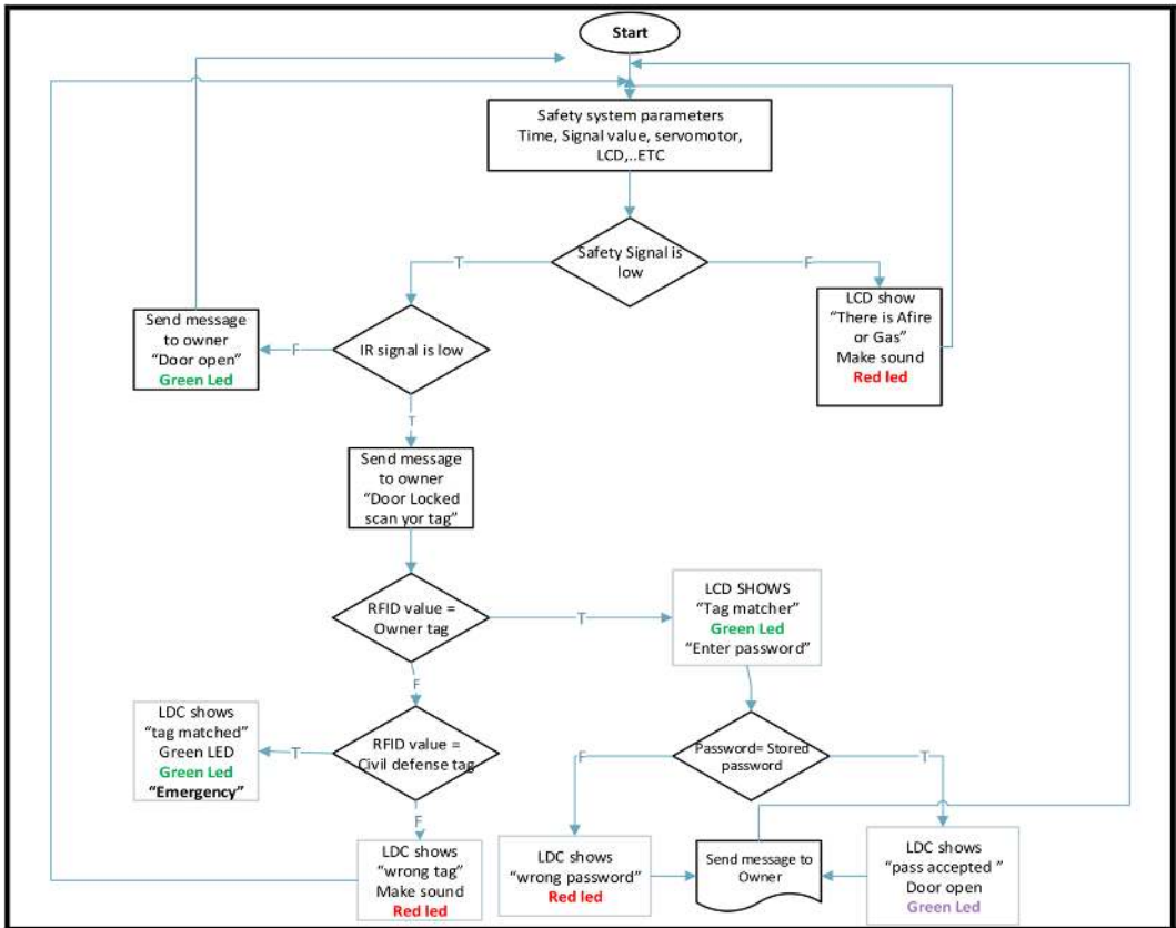
Figure 2. Safety and security system flowchart
