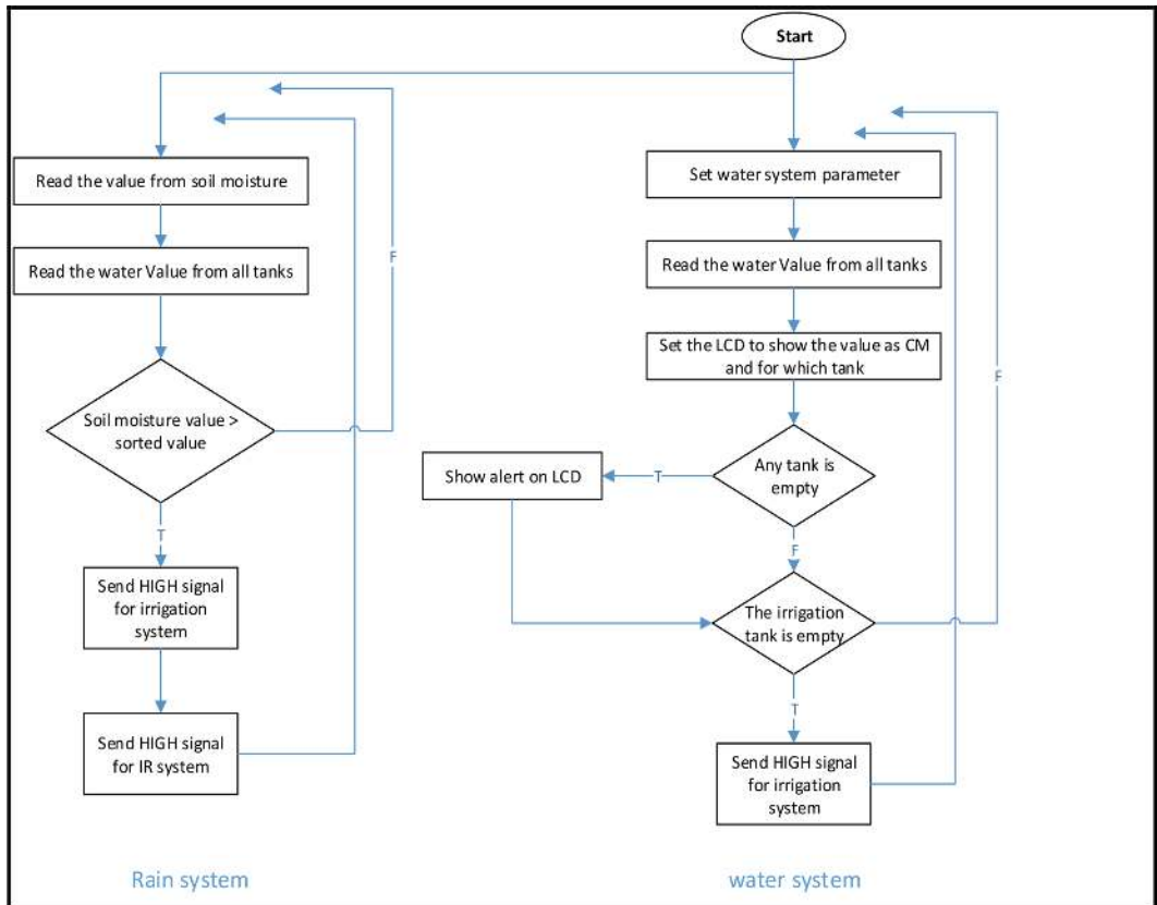
Figure 4. Water and rain system flowchart
