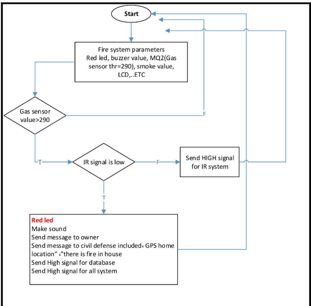
Figure 3. House Fire system flowchart
