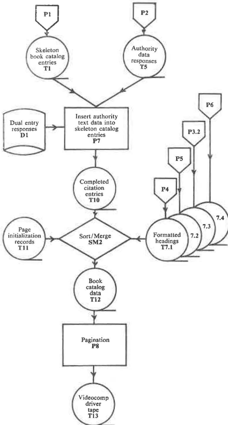
Fig. 10. Subsystem flow chart.
