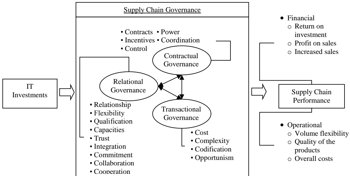
Figure 1. Proposed Model.
