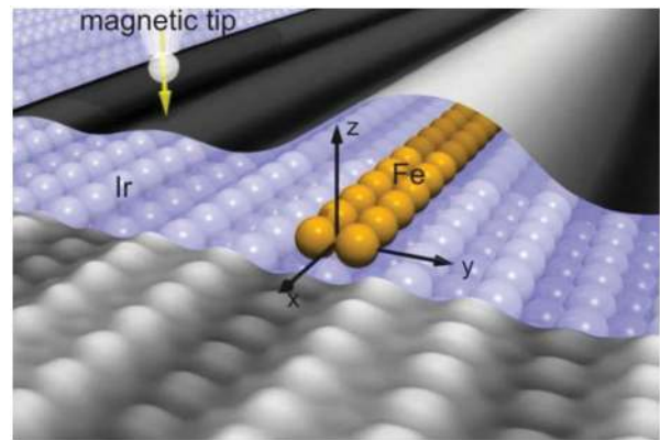
FIG. 1 (color). Schematic representation of the investigated sample system and the experimental setup. The STM image in the front shows the atomically resolved (5 \times 1) -reconstructed \text{Ir}(001) surface (measurement parameters: U = -2 mV, I = 40 nA, room temperature). Fe atoms deposited at room temperature form bi-atomic chains in the trenches of the reconstruction (ball model), which appear as a single strand in an STM image as shown in the overlaid image at the top (measurement parameters: U = +400 mV, I = 5 nA, T = 8 K). The experimental setup allows to apply magnetic fields perpendicular to the sample surface, i.e., along the z axis [10]. To investigate the magnetic order of the Fe chains we use spin-polarized STM with magnetic tips.
