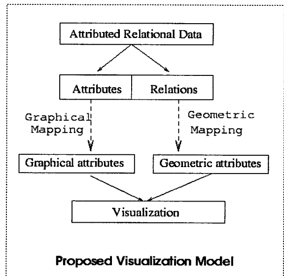
Figure 3.1: The Framework of Attributed Visualization.
