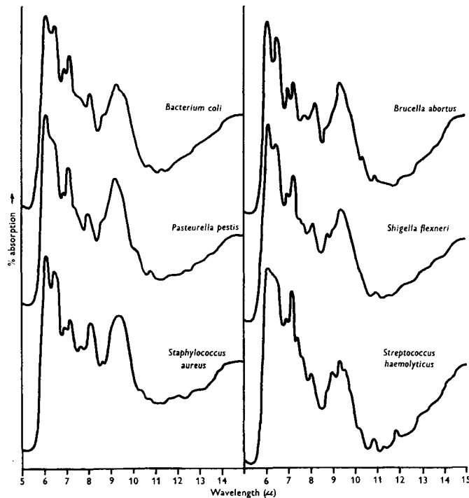
Fig. 2. Spectra typical of certain species of bacteria. (The spectra are displaced vertically.)
