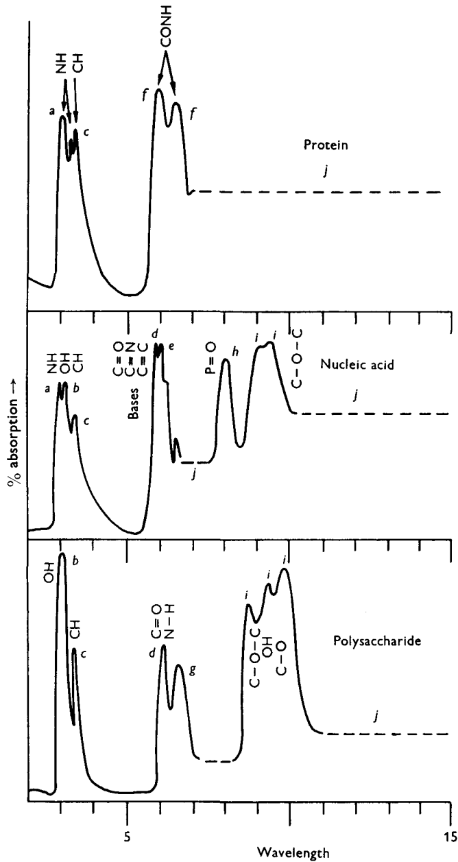
Fig. 1. Principal absorption bands in the spectra of protein, nucleic acid and polysaccharide. a , N-H stretching; b , O-H stretching; c , C-H stretching; d , C=O stretching; e , C=N and C=C of purine and pyrimidine bases; f , CONH vibrations of peptide link; g , N-H deformation in amino sugars; h , phosphorus vibrations; i , C-O-C vibrational modes, C-O stretching vibrations and OH deformation; j , regions of the spectrum which tend to be characteristic of the particular substance.
