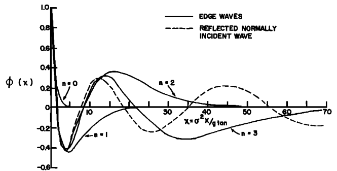
Fig. 1. Offshore dependence of edge waves of modes n = 0, 1, 2, 3 and of a reflected normally incident wave for a plane beach in terms of nondimensional offshore distance \chi = \sigma^2 x / g\beta .
