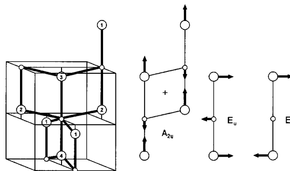
FIG. 1. The structure of the anatase primitive cell is shown at the left. The c axis is vertical, small circles denote Ti atoms, large circles denote O atoms. Oxygen atoms labeled with the same number are equivalent. The center figure shows (+) the position of the inversion center and the vibrational eigenvector for the A 2u mode. Symmetry coordinates for the E u modes are shown at the right.
