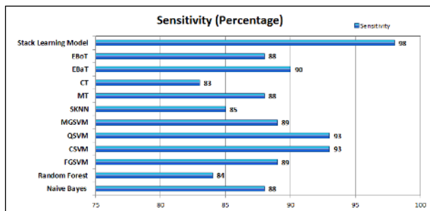
Fig. 8. Sensitivity of Classifiers using Different Machine Learning Algorithms
