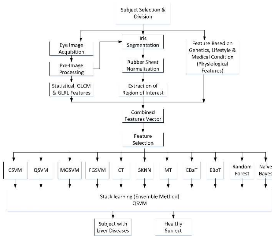
Fig. 1. Block Diagram of Infrared Sensing Based Non-invasive Initial Diagnosis of Chronic Liver Disease Using Ensemble Learning
