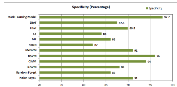
Fig. 9. Specificity of Classifiers for AI Based Non-invasive Diagnosis of Liver Disease
