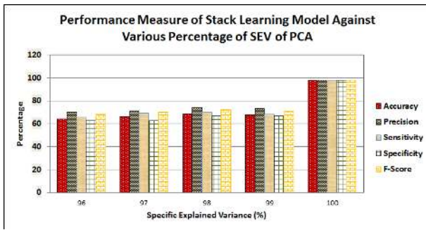
Fig. 4. Performance Measure of Stack Learning Model Against Various Percentage of SEV of PCA
