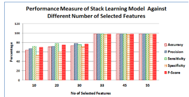
Fig. 5. Performance Measure of Stack Learning Model Against Different Number of Selected Features
