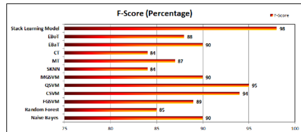
Fig. 10. F-Score Comparison of Different Classifiers.
