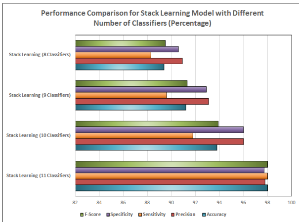
Fig. 12. Performance Comparison for Stack Learning Model with Different Number of Classifiers
