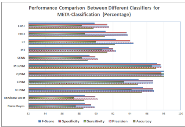
Fig. 11. Performance Comparison Between Different Classifiers for META-Classification
