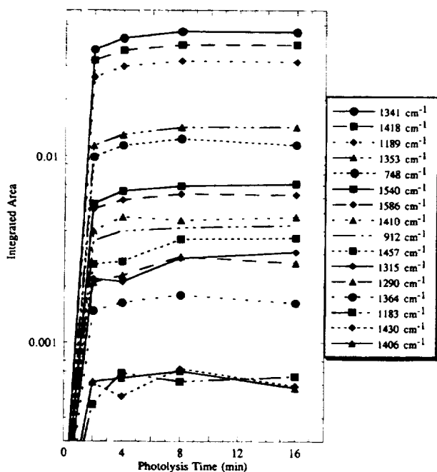
Figure 3. Growth of the anthracene cation integrated photoproduct band areas ( \text{cm}^{-1} ) as a function of photolysis time.
