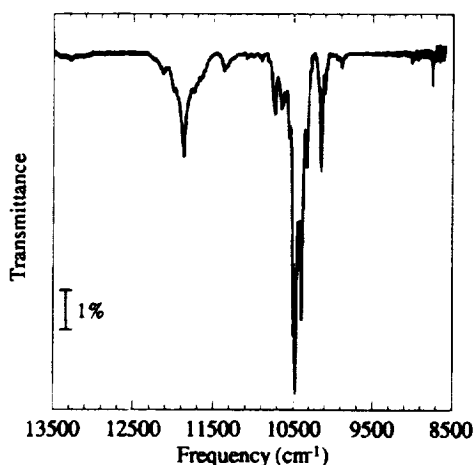
Figure 9. Near-infrared spectrum of the matrix isolated pentacene cation. This is of the same sample measured in the mid-infrared and shown in Figure 6 (argon matrix, 10 K).
