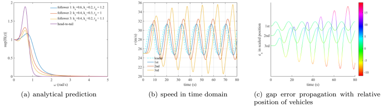
Figure 7: Example 3: string instability of heterogeneous platoon under periodic leader disturbance
