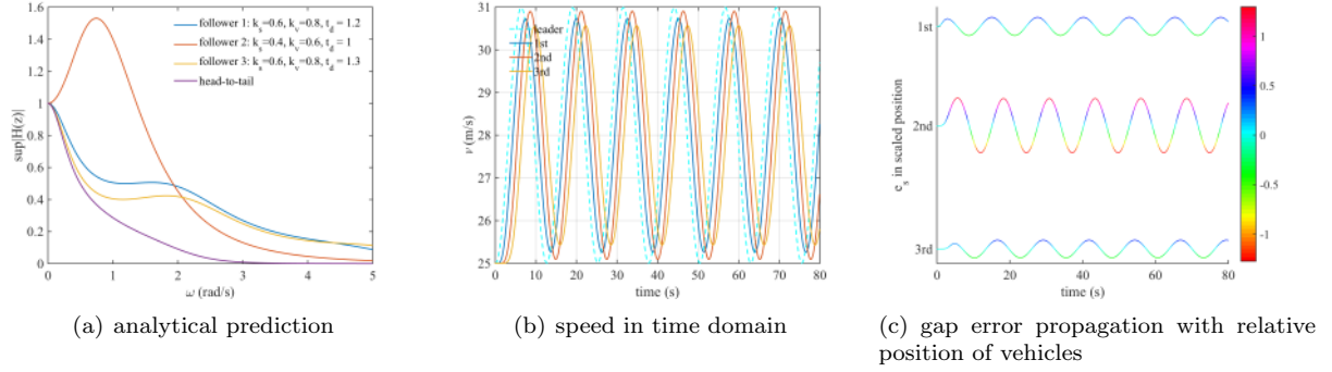
Figure 6: Example 2: weak/head-to-tail string stability of heterogeneous platoon under periodic leader disturbance
