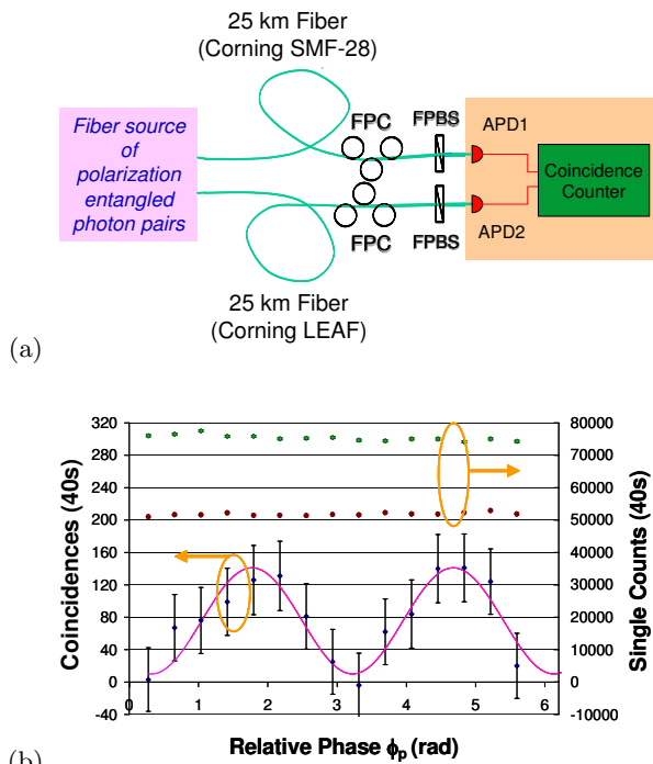
Figure 9: (a): Schematic of the experimental setup to demonstrate long-distance entanglement distribution. FPC, fiber polarization controller; FPBS, fiber-pigtailed polarization beam splitter; APD, avalanche-photodiode based photon-counting detector. (b): Single counts (right ordinate) and coincidence counts (left ordinate) registered by the detectors of Stokes and anti-Stokes photons versus the relative phase between the source’s two pump pulses. The contribution of accidental coincidences has been subtracted.
