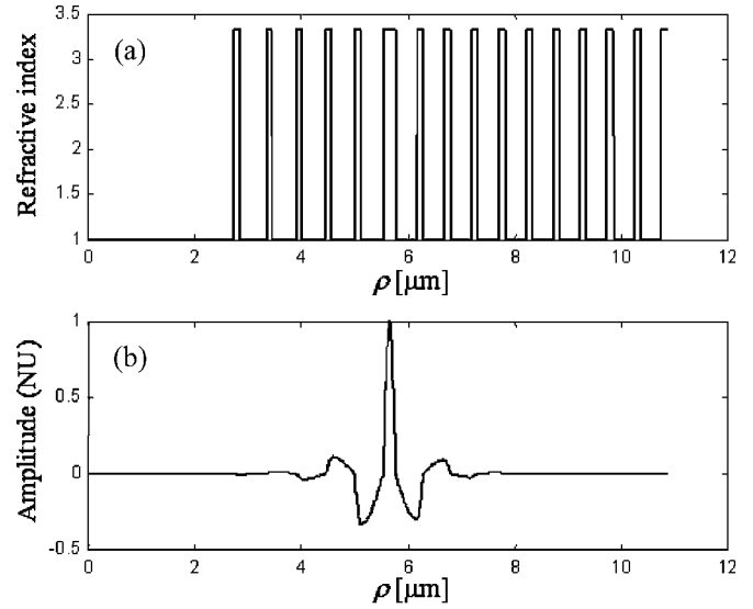
Fig. 2. (a) Refractive index and (b) TE-polarized modal field profiles of an ABR designed for m = 7 , \lambda_{\text{res}} = 0.852 \mu\text{m} , with five internal and ten external Bragg layers.
