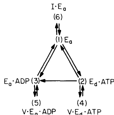
FIGURE 9 A kinetic model for the flagellar ATP-dephosphorylation cycle. E_a , dynein ATPase of attached state; E_d , detached state; ATP , MgATP^{2-} ; ADP , MgADP^- ; V , vanadate; I , any of several competitive inhibitors, such as ATP^{4-} , ADP^{3-} , or P_i .
