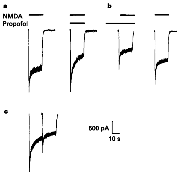
Figure 4 The inhibition of currents evoked by NMDA does not demonstrate the features typical of a use-dependent block. (a) Under control conditions, a 20 s application of NMDA ( 50 \mu\text{M} ) activated a current which rapidly reached a peak and then declined. The second trace demonstrates the response to a co-application of propofol ( 600 \mu\text{M} ). The peak current was decreased by 4% whereas the nondesensitized component, measured at the end of the application, was decreased by 37%. (b) Pre-application of 600 \mu\text{M} propofol reduced the peak and quasi steady-state response by 46% and 49%, respectively. A subsequent application of NMDA alone generated a peak response which recovered to 80% of the control value. (c) Currents recorded during the co-application (a, second trace) or following pre-exposure to propofol (b, first trace) are shown superimposed upon each other. These data suggest that the rate of current decay is similar regardless of the method of application of propofol.
