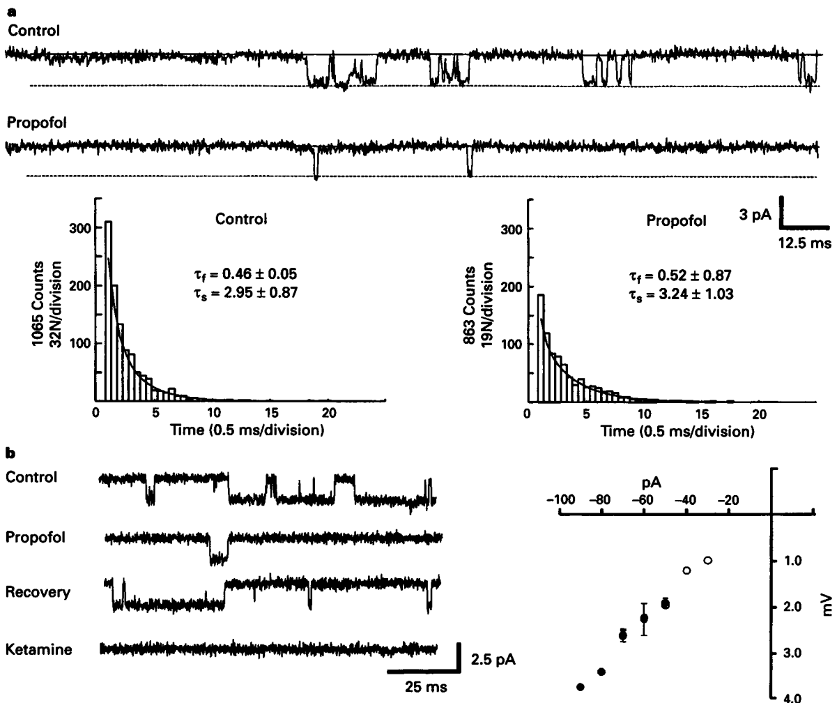
Figure 7 Propofol reduces the frequency of NMDA channel opening. (a) An example of single channel currents from an outside-out patch. The pipette solution contained \text{Cs}_2\text{SO}_4 and the patch was voltage clamped at -70 mV. Traces represent current low pass filtered at 2 kHz ( -3 dB) and digitized at 0.1 ms/point. Inward current is represented by a downward deflection and the closed and open states are indicated by the solid and dashed lines respectively. The addition of 100 \mu\text{M} propofol to the perfusate containing 10 \mu\text{M} NMDA, caused a reversible decrease in frequency of channel opening. The open duration histograms for the control and propofol currents are indicated below the tracings. The time constants for the illustrated control and propofol curves were \tau_f = 0.75 ms, \tau_s = 2.43 ms, and \tau_f = 0.43 , \tau_s = 2.94 , respectively. Propofol had no apparent effect on the fast ( \tau_f ) or slow ( \tau_s ) time constants. (b) Currents from a different patch, voltage-clamped at -50 mV, recorded in the absence and presence of propofol are shown. Ketamine ( 20 \mu\text{M} ), added to the bath solution abolished residual open events providing further confirmation of the identity of the channels. The I-V plot for single channel currents activated by 10 \mu\text{M} NMDA revealed a slope-conductance of 47 pS and 45 pS for currents recorded in the absence ( \bullet ) and presence ( \circ ) of 100 \mu\text{M} propofol. The mean current amplitudes \pm s.e.mean are shown ( n = 5 patches).
