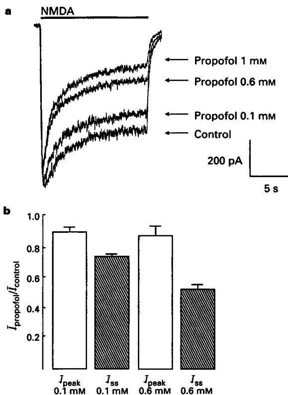
Figure 1 Propofol inhibition of NMDA-activated currents recorded from hippocampal neurones. (a) Representative traces of currents evoked by NMDA ( 50 \mu\text{M} ), in the absence or presence of propofol are shown. Traces are superimposed upon each other and the period of perfusion is indicated by the horizontal bar at the top of the traces. Propofol caused a concentration-dependent reduction in the amplitude of these currents. Note that the steady-state component is reduced to a greater extent than the peak response. (b) The fractional reduction of peak ( I_{\text{peak}} ) and steady-state currents ( I_{\text{ss}} ), recorded in the presence of propofol 0.1 \text{mM} ( n=6 ) and 0.6 \text{mM} ( n=5 ) is illustrated. Neurones were voltage-clamped at a holding potential of -65 \text{mV} .
