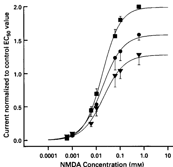
Figure 6 Concentration-response curves for peak NMDA-evoked currents recorded in the presence or absence of propofol. Neurons were voltage clamped at -65\text{mV} and currents were activated by applying NMDA ( 0.6 \mu\text{M} - 1 \text{mM} ). Cells were exposed to propofol ( 30 \mu\text{M} or 100 \mu\text{M} ) and NMDA was re-applied. Paired dose-response curves were constructed and responses normalized to the concentration of NMDA that evoked the half-maximal response ( \text{EC}_{50} ) under control conditions. The ordinate scale indicates peak responses normalized to the NMDA \text{EC}_{50} value for individual neurons and the abscissa scale shows the concentration of NMDA ( \mu\text{M} ). The apparent affinity of the receptor for NMDA ( K_d ) and Hill coefficients ( n_H ) for the various recording conditions were determined by fitting the curves to a standard logistic equation. No significant differences observed in the absence (■) or presence of propofol 100 \mu\text{M} (▼), 30 \mu\text{M} (●), for the K_d : 20.6 \pm 3.4 \mu\text{M} ( n=9 ), 19.9 \pm 2.88 \mu\text{M} ( n=5 ), 24.0 \pm 10.2 \mu\text{M} ( n=4 ), respectively, or n_H values: 1.24 \pm 0.06 , 1.38 \pm 0.16 , 1.31 \pm 0.31 , ( P > 0.05 Student's t test).
