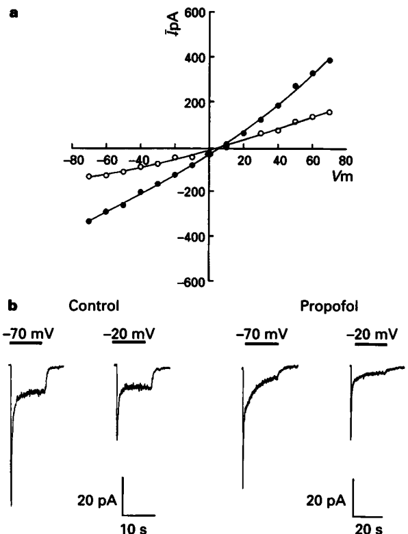
Figure 5 Propofol inhibition of NMDA-evoked currents is independent of membrane potential. (a) Current-voltage relation for responses activated by 100 \mu\text{M} NMDA were recorded in the absence (●) or presence (○) of propofol ( 600 \mu\text{M} ). Cells were voltage clamped at -65 \text{ mV} and exposed to a prolonged application of agonist. Currents were observed to peak and then decline to an apparent steady-state. Once a stable current level was reached, the membrane potential was adjusted in 10 \text{ mV} steps ranging from -70 \text{ mV} to +70 \text{ mV} for 100 \text{ ms} and the steady-state current recorded. The cell was then voltage clamped at -65 \text{ mV} and NMDA washed away. This protocol was repeated in the presence of NMDA plus propofol ( 600 \mu\text{M} ). In addition, the amplitude of currents activated by propofol ( 600 \mu\text{M} ) alone was measured at the various holding potentials and subtracted from the NMDA plus propofol current records. The I-V plot illustrates the amplitude of the steady-state responses. Leak and capacitance currents, measured in the absence of agonist and propofol were also subtracted from the records. NMDA-evoked currents were depressed equally at hyperpolarizing and depolarizing potentials: propofol reduced responses to 40% of control at -70 \text{ mV} and +70 \text{ mV} . (b) In a different cell, the voltage-dependence of block by propofol was further investigated. Cells were voltage-clamped at -70 \text{ mV} or -20 \text{ mV} and NMDA, or NMDA plus propofol, applied for 10 \text{ s} . Propofol ( 1 \text{ mM} ) was seen to reduce the amplitude of the steady-state response to 42% of control, at both holding potentials.
