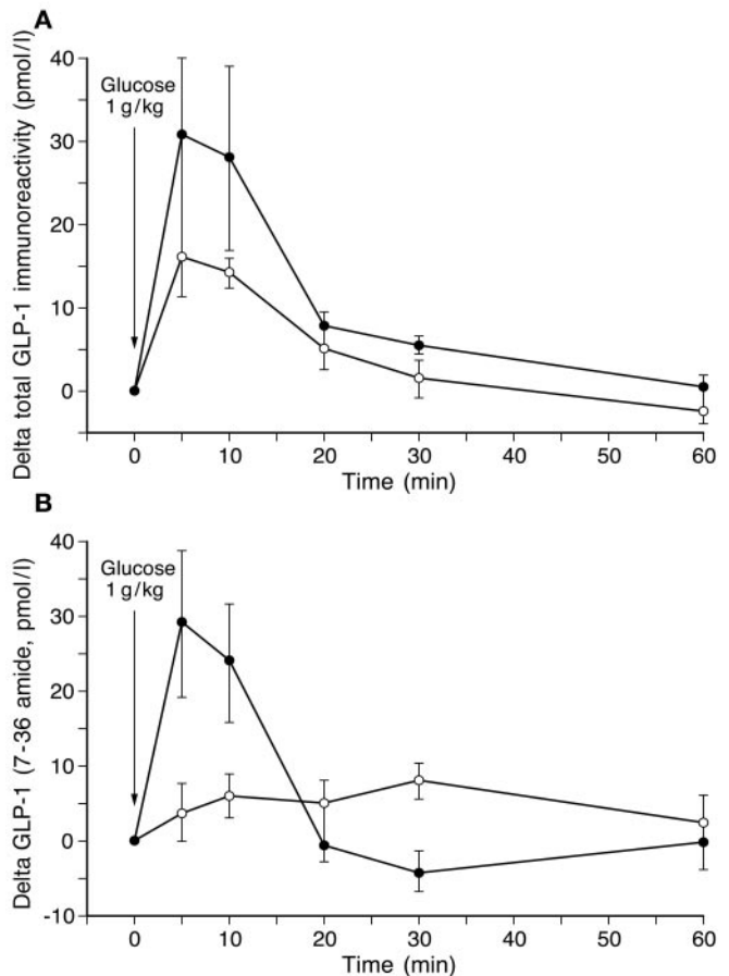
Fig. 5 A, B. Changes in plasma immunoreactive GLP-1 (7–36) amide (A) and total plasma GLP-1 immunoreactivity (B) during an oral glucose tolerance test in obese ( fa/fa ) Zucker rats ( n=8 ) after vehicle (CMC) or compound (NVP-DPP728, 10 \mu\text{mol/kg} ) given at -30 min. All animals received 1 g/kg glucose orally at 0 min. The data are displayed as means \pm SEM of individual delta plasma GLP-1 concentrations from basal (pre-glucose, 0 min.) levels. —○— vehicle —●— NVP-DPP728
