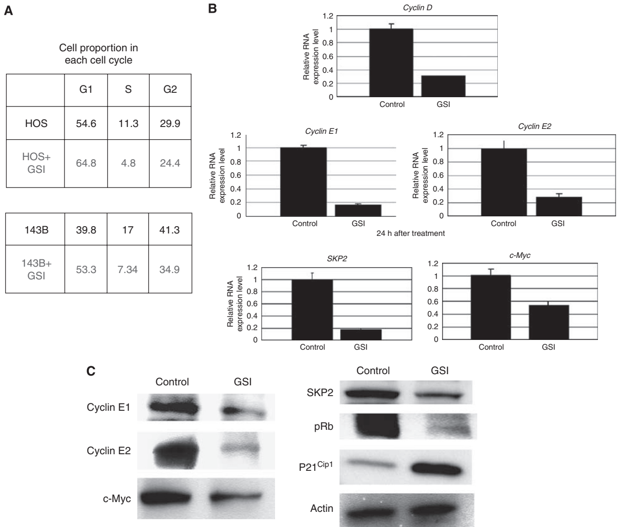
Figure 4 Notch pathway inhibition promotes G1 arrest. HOS and 143B cells were treated with 5 \mu\text{M} GSI. After 48-h treatment, cells were collected and subjected to cell cycle analysis. When HOS cells were cultured without GSI, 54.6% of cells were in G1 phase. On the other hand, when cultured with GSI, 64.8% of cells were in G1 phase. In the case of 143B cells cultured without GSI, 39.8% of cells were in G1 phase, whereas 53.3% of cells were in G1 phase when treated with GSI ( A ). Real-time PCR was carried out to quantify mRNAs of cell cycle-related genes. A 24-h treatment with GSI reduced the levels of cyclin D , cyclin E1 , E2 , SKP2 , and c-Myc transcription (error bar means s.d.; B ). Western blot analysis of the levels of cell cycle-related genes. 48 h treatment with GSI reduced the levels of expression of cyclin E1, cyclin E2, c-Myc, pRb, and SKP2 proteins. Expression of P21 Cip1 protein was upregulated by GSI treatment. The experiment was triplicate with similar results ( C ; GSI: 5 \mu\text{M} ).
