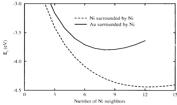
FIG. 3. The E_c function plotted as a function of coordination number N for a Ni atom and for a Au atom, in both cases surrounded by Ni neighbors at the equilibrium Ni bulk nearest-neighbor distance.
