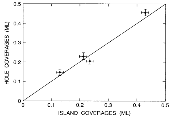
FIG. 2. The density of the Au induced holes in ML, counted from STM topographs with atomic resolution, as a function of the density of 2D Ni islands, measured from height distributions of large area STM topographs as depicted in Fig. 1(c). The solid line corresponds to equal hole and island coverages.
