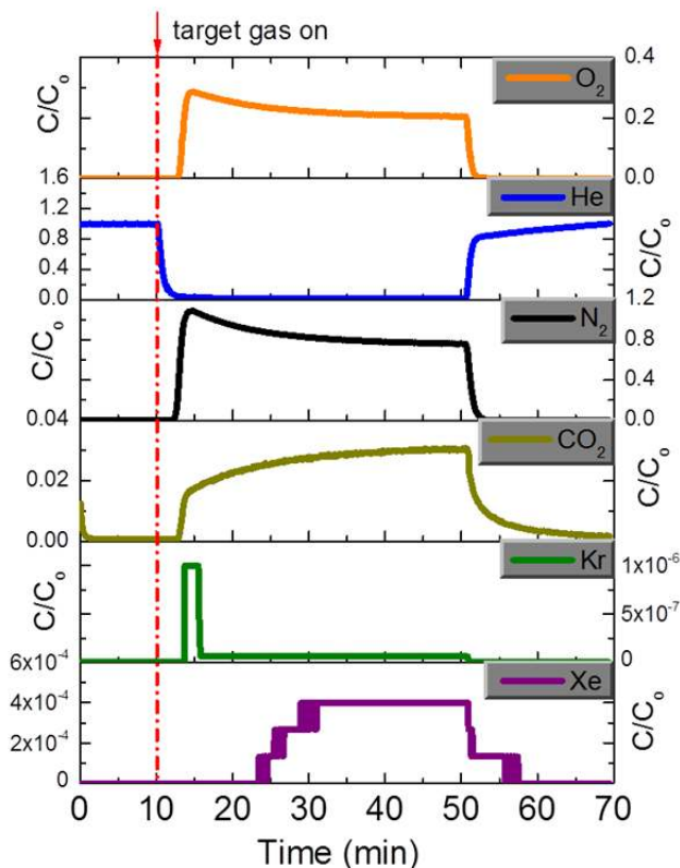
Figure 6. Xenon 400 ppmv and Kr 40 ppmv in air breakthrough curves at 25 °C for the Ni/DOBDC. The flow rates are 20 scfm.
