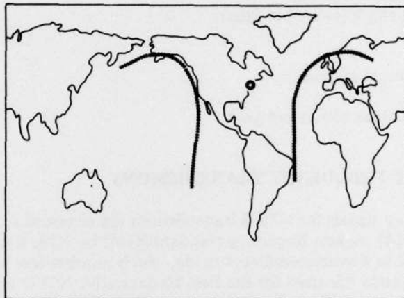
Fig. 12 - Chesapeake Bay Division NTS-2 coverage
