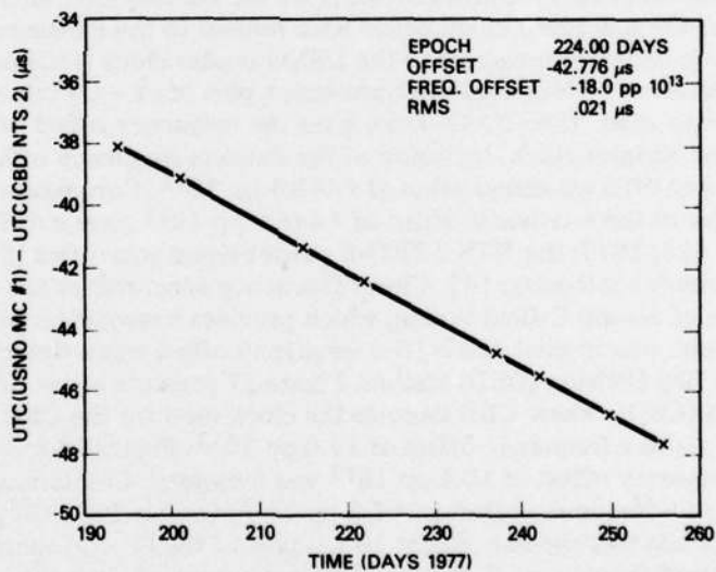
Fig. 17 — Frequency offset determined by the clock rate between the CBD clock and the USNO clock: USNO - CBD
