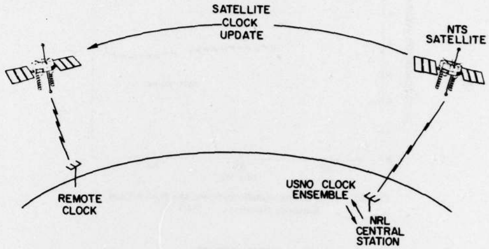
Fig. 21 — Technique of time transfer by the navigation-technology segment of the NAVSTAR GPS
