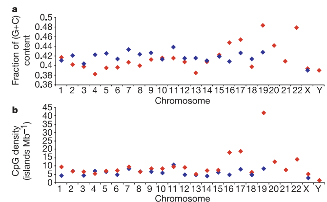
Figure 8 (G+C) content and density of CpG islands shows more variability in human (red) than mouse (blue) chromosomes. a , The (G+C) content for each of the mouse chromosomes is relatively similar, whereas human chromosomes show more variation; chromosomes 16, 17, 19 and 22 have higher (G+C) content, and chromosome 13 lower (G+C) content. b , Similarly, the density of CpG islands is relatively homogenous for all mouse chromosomes and more variable in human, with the same exceptions. Note that the mouse and human chromosomes are matched by chromosome number, not by regions of conserved synteny.
