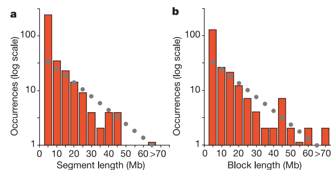
Figure 5 Size distribution of segments and blocks with syntenic conservation between mouse and human. a, b, The number of segments (a) and blocks (b) with syntenic conservation between mouse and human in 5-Mb bins (starting with 0.3–5 Mb) is plotted on a logarithmic scale. The dots indicate the expected values for the exponential curve of random breakage given the number of blocks and segments, respectively.
