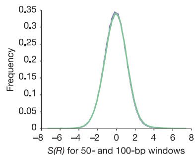
Figure 23 Distribution of the conservation score S(R) . The empirical distribution of S(R) for all 1.9 million non-overlapping 50-bp windows (blue) containing at least 45 aligned ancestral repeat sites (standard deviation 1.19) and 1.7 million non-overlapping 100-bp windows (green) containing at least 50 aligned ancestral repeat sites (standard deviation 1.23). Both curves are bell-shaped, with a mean of zero, but the standard deviations are higher than would be expected if the sites in each window were independent and conserved with (locally estimated) probability \mu . In that case the distribution of S would be approximately normal with a standard deviation of 1. Thus, these data show that there is some dependency between the substitutions within the window.
