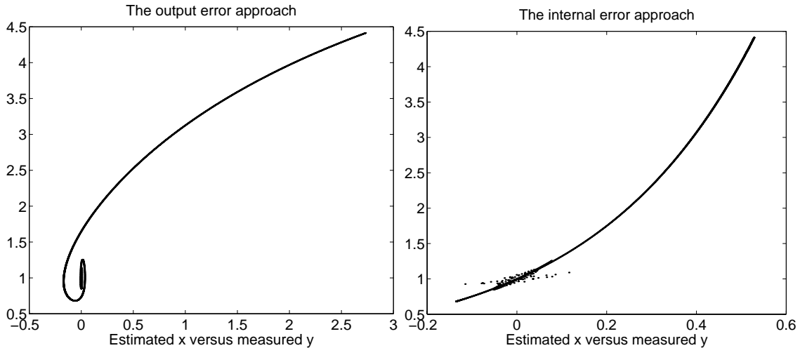
Figure 2: Example of initial estimates with non-Gaussian input. The output error approach is to the left and the internal error approach to the right.
