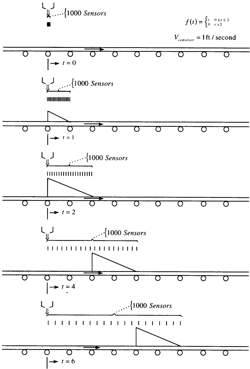
Figure 3-2-3(a).—Conveyer analogy: Fixed N , here n = 1000 , sensors uniformly spread between 0 and t , spacing varies with t .
