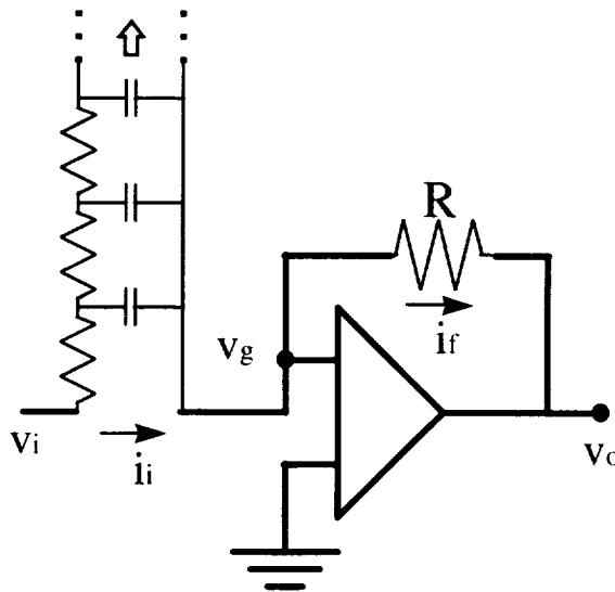
Figure 7-5-2.—Semi-differentiator.
