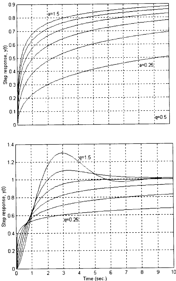
Figure 7-10-1.—Fractional order tracking filter response to unit step input, varying q ( a = 1 ) and varying a ( q = 0.5 ).
