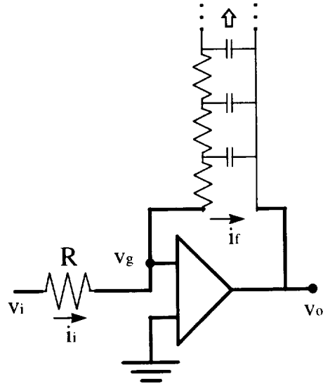
Figure 7-5-1.—Semi-integrator.
