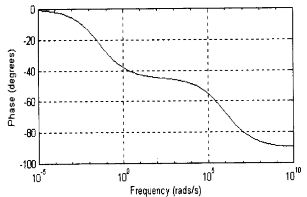
Figure 7-7-2.—Frequency response of dynamic thermocouple.
