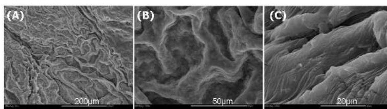
Fig. 2. The SEM images of dendrimer [(\text{NH}_2)_{49}\text{-G4-(NH-PDP)}_{15}] crosslinked with 8-PEG-SH gel (A) 200 μm (200x) (B) 50 μm (1000x) (C) 20 μm (2000x). These gels were dehydrated by lyophilization.
