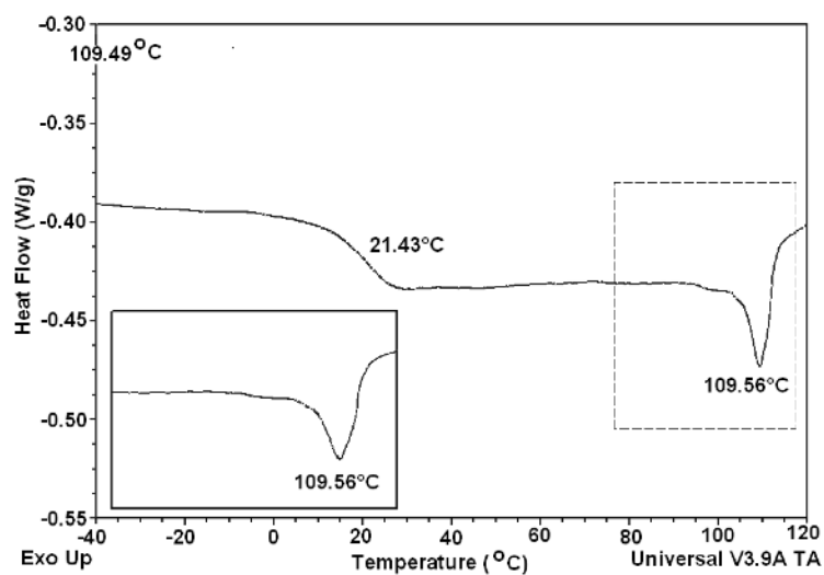
Fig. 1. The DSC thermogram of [(\text{NH}_2)_{49}\text{-G4}\text{-(NH-PDP)}_{15}] shows the T_g at 21.4^\circ\text{C} and an endotherm at 109.6^\circ\text{C} . The increase in T_g to 21.4^\circ\text{C} from -28^\circ\text{C} indicates modification of amine terminated PAMAM dendrimer with PDP groups.
