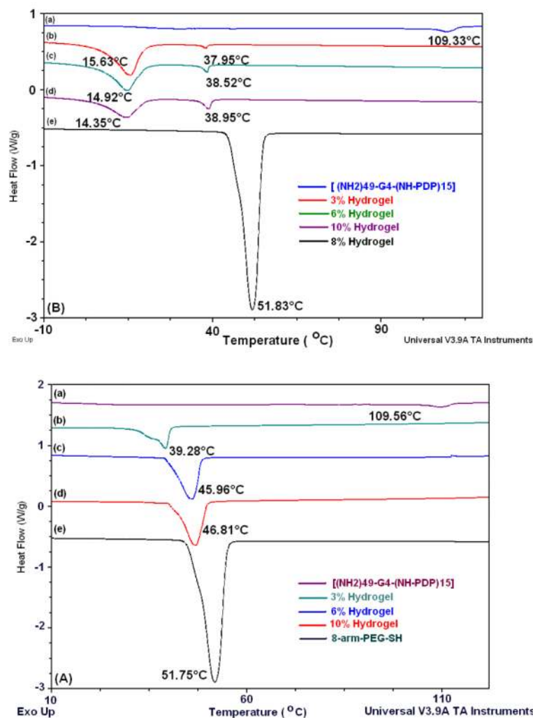
Fig. 4. The DSC thermograms for the 3, 6 and 10 % dendrimer-PEG hydrogels. (A) Hydrogels without formulation additives (absence of glycerin, PVP and PEG600), The 8-arm-PEG-SH (e) shows an endotherm at 51.7°C, which is lowered on crosslinking with [(NH 2 ) 49 -G 4 -(NH-PDP) 15 ] as seen in curves (b), (c) and (d) for 3, 6 and 10% hydrogels respectively (B) Hydrogels with formulation additives (glycerin, PVP and PEG 600). In addition to the endotherms corresponding to 8-arm-PEG-SH (37.9 to 38.9°C) in hydrogels, an endotherm for PEG 600 is seen between 15.6 to 14.3 °C.
