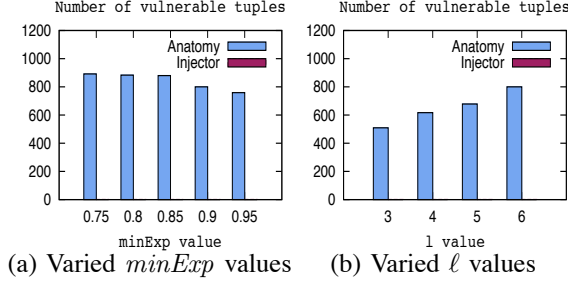
Fig. 4. Background knowledge attack
