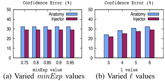
Fig. 6. Confidence error
