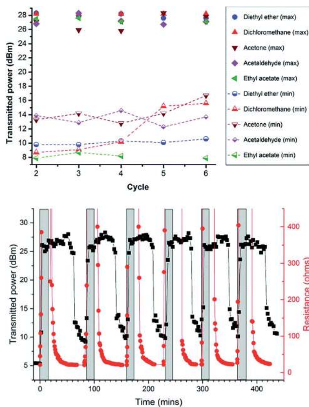
Fig. 24 (Top) Silver inkjet-printed RFID tag sensors used for detecting a variety of VOCs. Silver ink used in inkjet printing onto PDMS substrates showing maximum (max) and minimum (min) transmitted power per cycle for organic solvents. (Lower) Measured transmitted power and electrical resistance as a function of time for silver inkjet printed RFID tag for diethyl ether vapors. The grey box shows the loop exposure time to diethyl ether vapor. [Reprinted with permission from ref. 254 Copyright © The Royal Society of Chemistry.]
