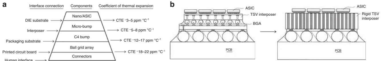
Figure 1 (a) Interface pyramid showing the components in a conventional package, along with the estimated CTEs of the involved substrates. (b) Introducing a rigid 3D TSV interposer (right) to bridge the mismatch of the CTE values of the PCB board and the Si application-specific integrated circuit (ASIC) dies 3 . CTE, coefficients of thermal expansion; PCB, printed circuit boards; 3D TSV, three dimensional through silicon via.
