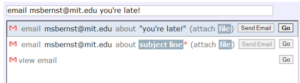
Figure 4: Commands can be run in either view mode (Go) or submit mode (e.g., Send Email).
