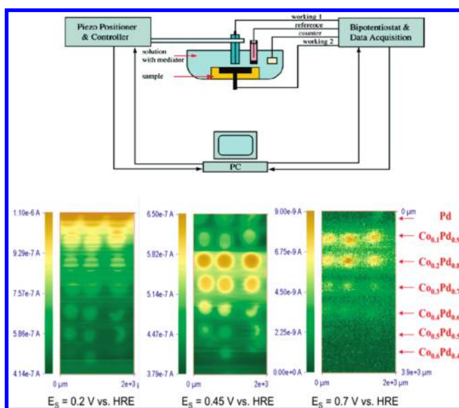
Figure 6. Top: Schematic diagram of a scanning electrochemical microscope and tip (working electrode 1) scanning above the array (sample) (working electrode 2). Bottom: Results for scanning an array of Pd–Co spots (indicated at right) in a solution of deaerated 0.5 M \text{H}_2\text{SO}_4 held at different potentials, where the tip generates \text{O}_2 as it scans across the array. Each row is a replicate of three spots to indicate reproducibility in spot preparation. Adapted with permission from ref 24. Copyright 2005 American Chemical Society.
