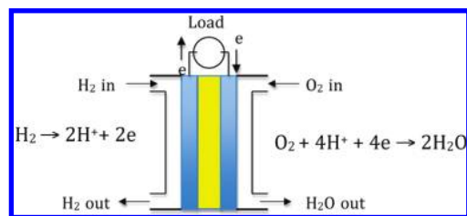
Figure 1. Schematic of polymer membrane electrolyte hydrogen–oxygen fuel cell.
