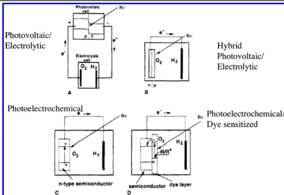
Figure 7. Schematic diagram of different types of photoelectrochemical cells. Adapted with permission from ref 38. Copyright 1995 American Chemical Society.
